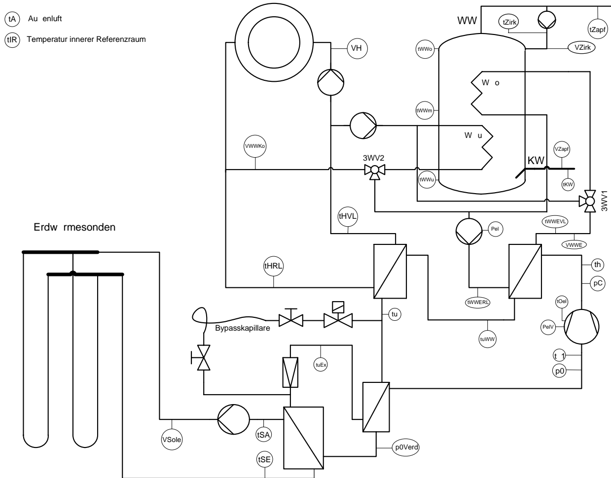
Fig. 3. Schematic of the Heat Pump System
