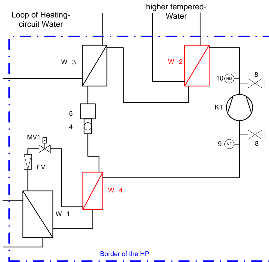
Fig. 2. Schematic of the Heat Pump Circuit
