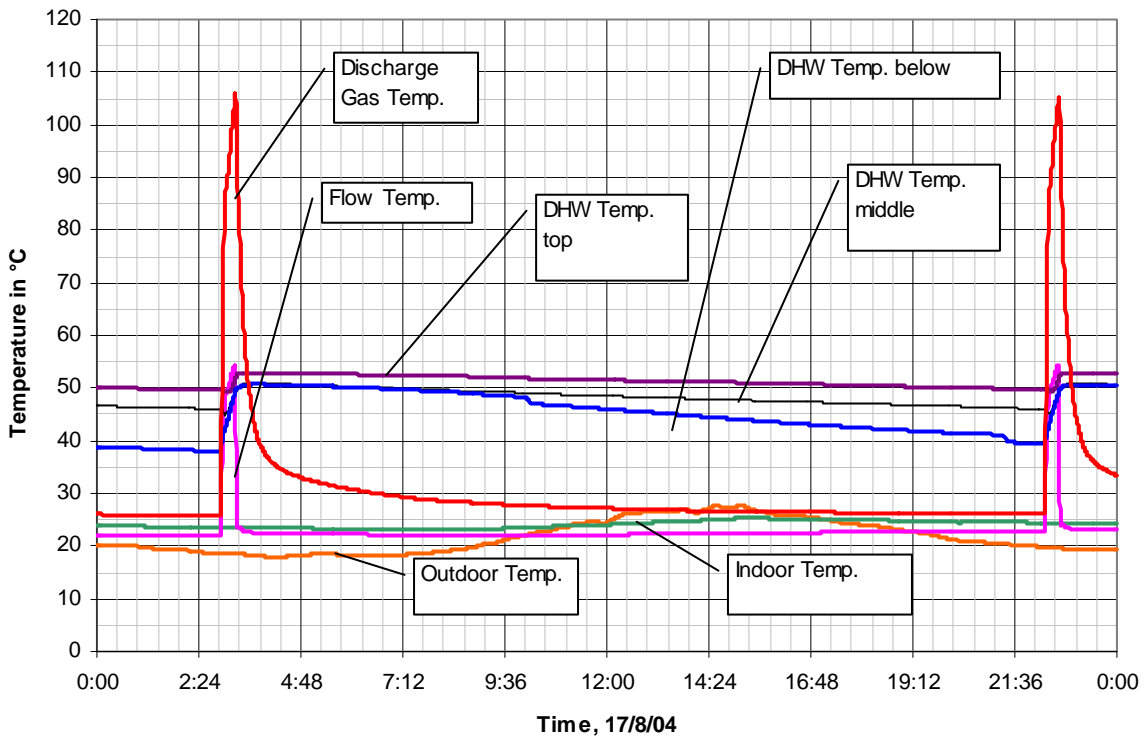
Fig. 5. Typical behaviour on a summer day
