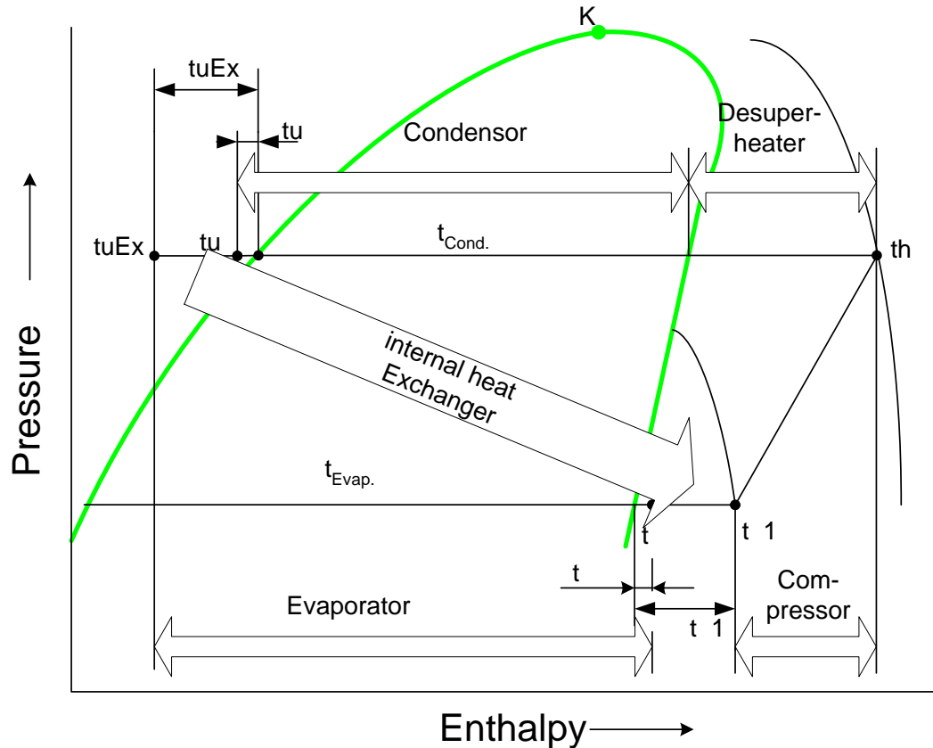
Fig. 1. Logarithmic Pressure, Enthalpy- Diagram
