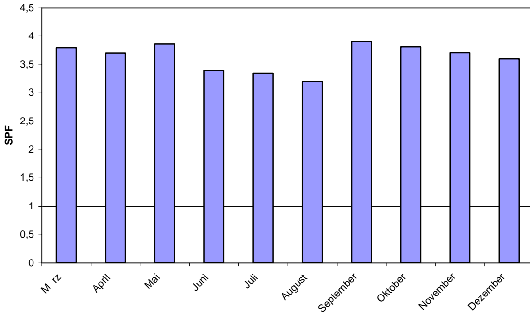
Fig. 7. Seasonal Performance Factor of the installation
