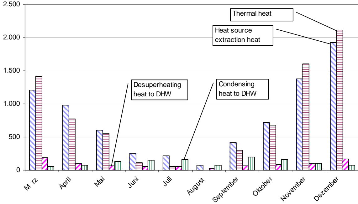
Fig. 6. Amounts of heat per month in kWh
