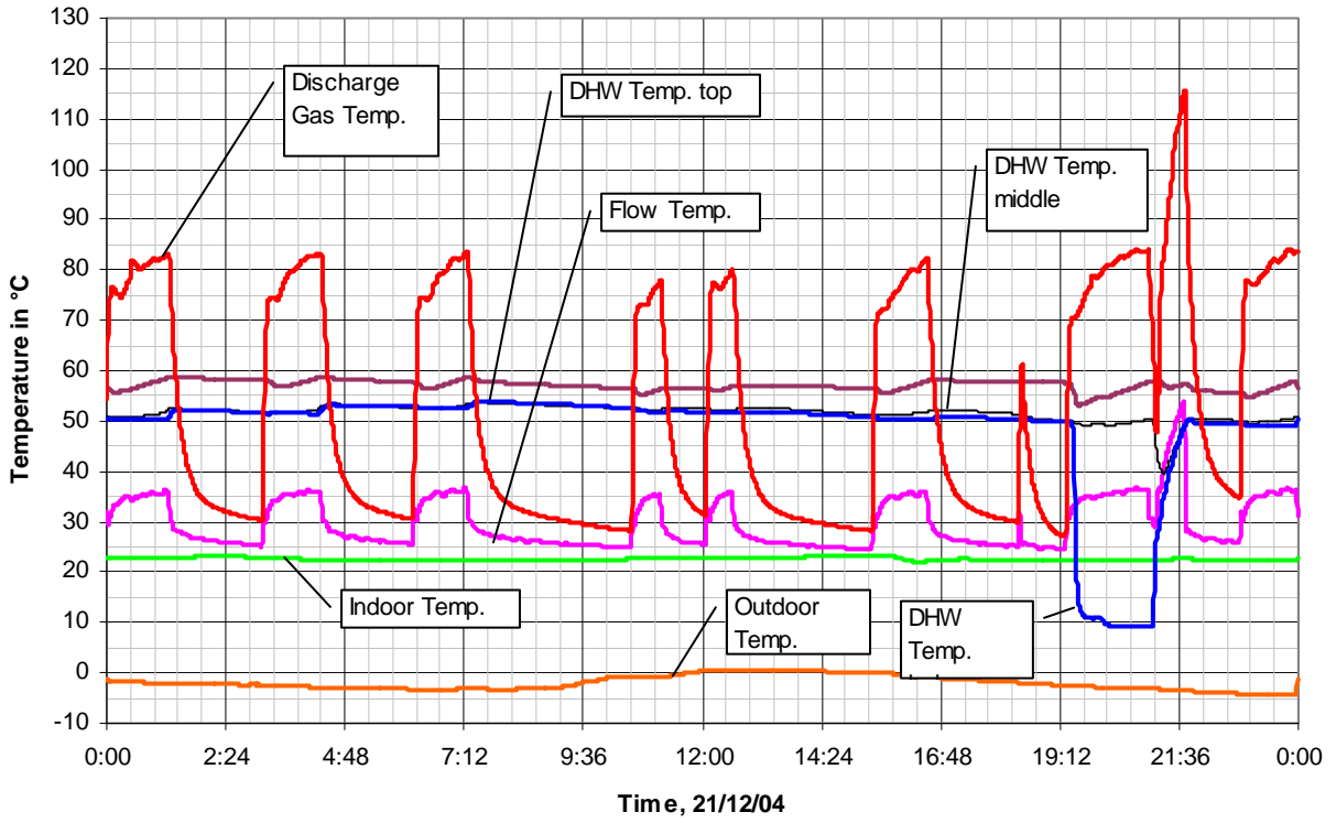
Fig. 4. Typical behaviour on a winter day
