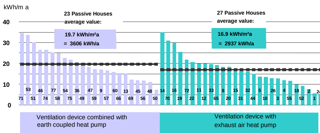
Fig. 8. Results of the field test of Passive Houses with electrical driven heat pump and a thermal solar collector. Every bar shows the yearly electrical energy demand of HVAC, related to the heated floor area of the building. The systems with exhaust air heat pump shows in average a higher performance than the earth coupled heat pump systems.
