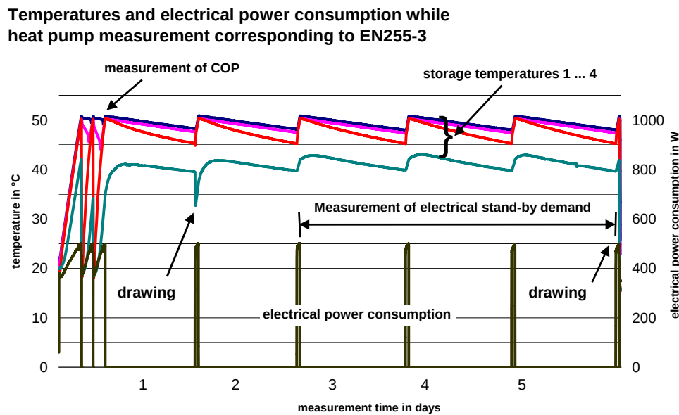
Fig. 4. Test procedure as defined in EN 255-3
