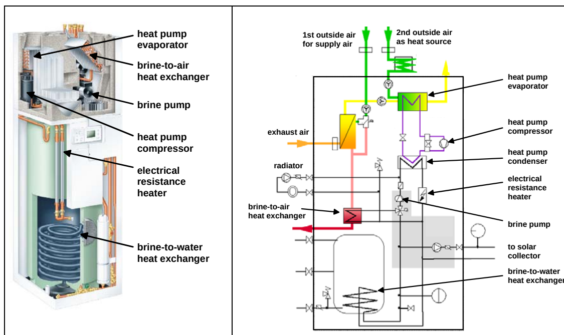
Fig. 7. Design and scheme of system C with internal brine loop.
