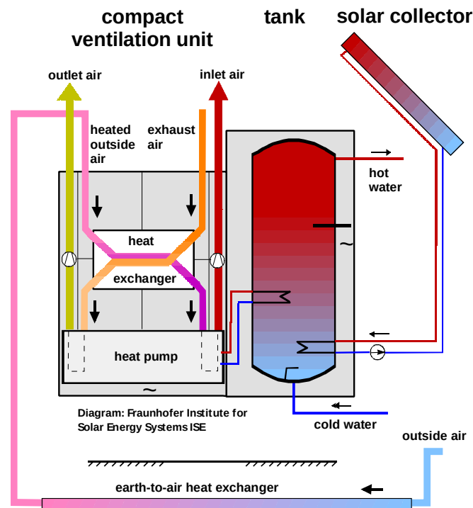
Fig. 2. System concept of a compact ventilation and heating device with integrated exhaust air heat pump to supply passive houses with space heat, domestic hot water and fresh air.
