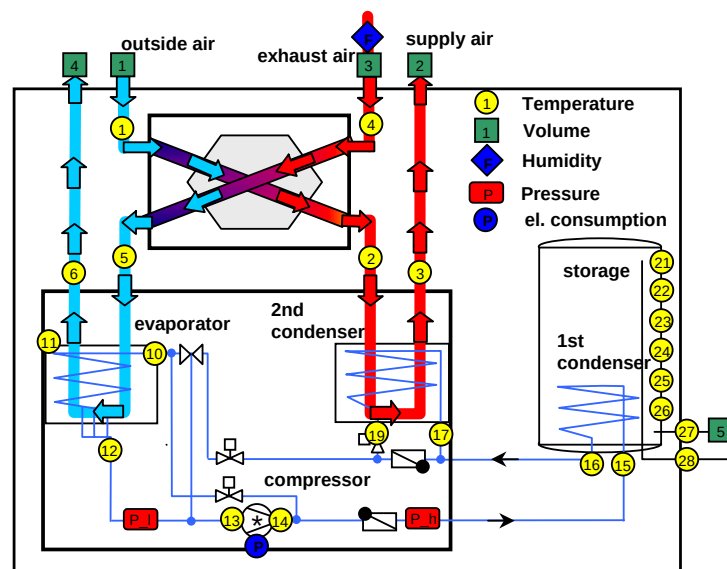
Fig. 6. Design and scheme of system B with two condensers in series. All sensors were used for the measurements at the test facility to quantify not only overall system efficiency but also component performance.
