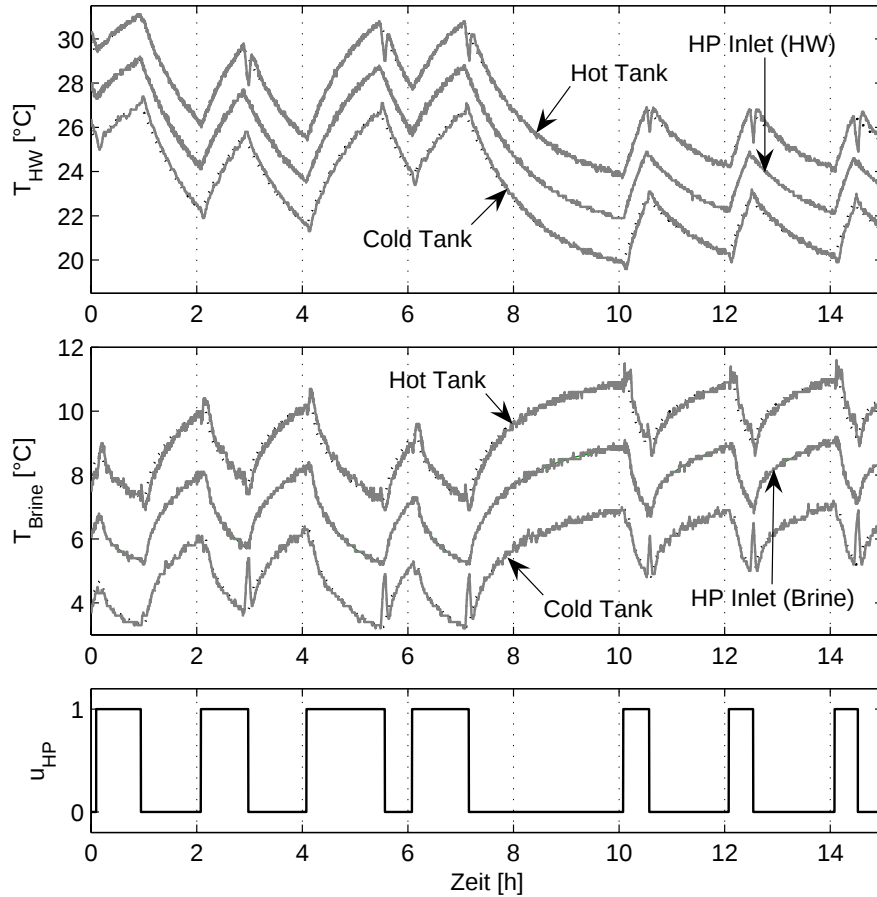
Fig. 6. Short test of a dynamic emulation.
