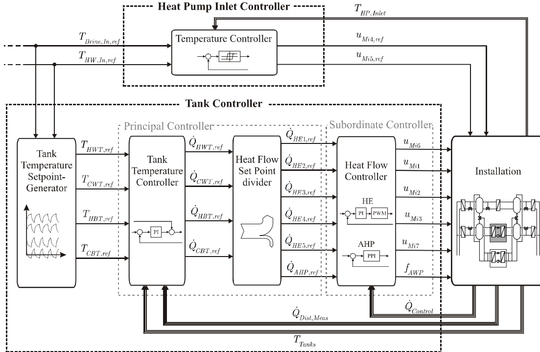
Fig. 4. Overview of the test bench controller.
