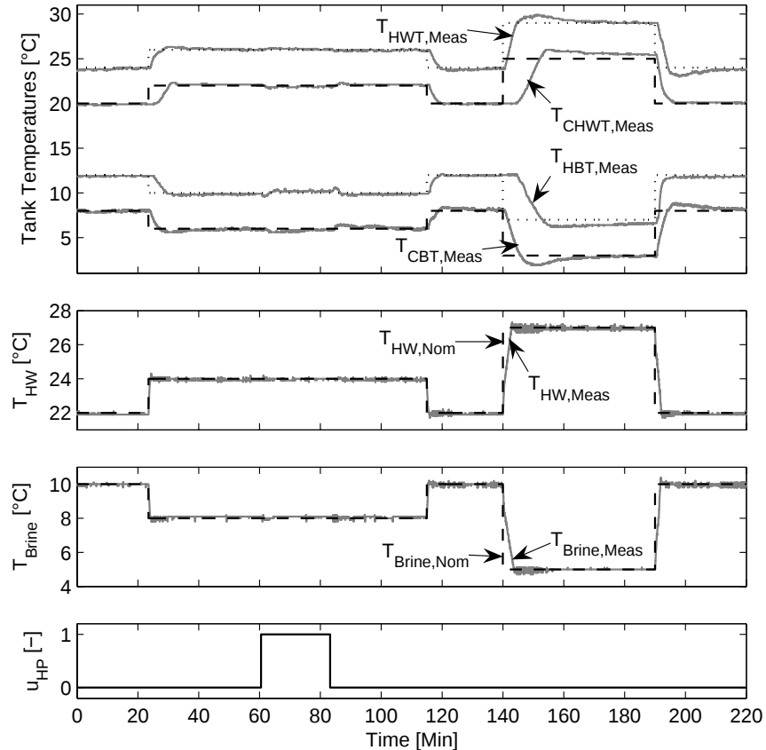
Fig. 5. Response of the test bench to excitations.
