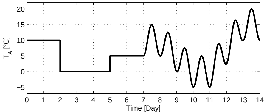
Fig. 7. Outdoor temperature course for the controller comparison.
