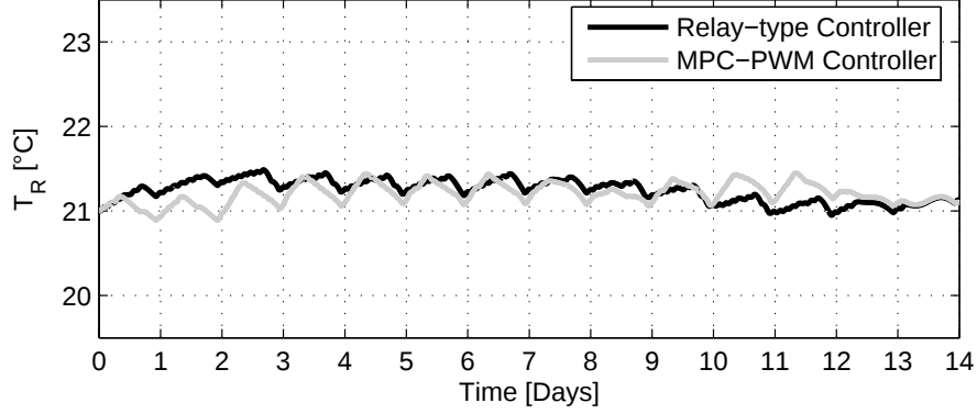
Fig. 8. Emulated room temperature course for the two controllers tested.
