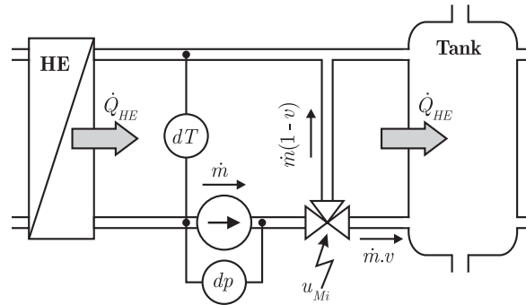
Fig. 3. Detailed illustration of the heat flow exchange between heat exchanger and tank.
