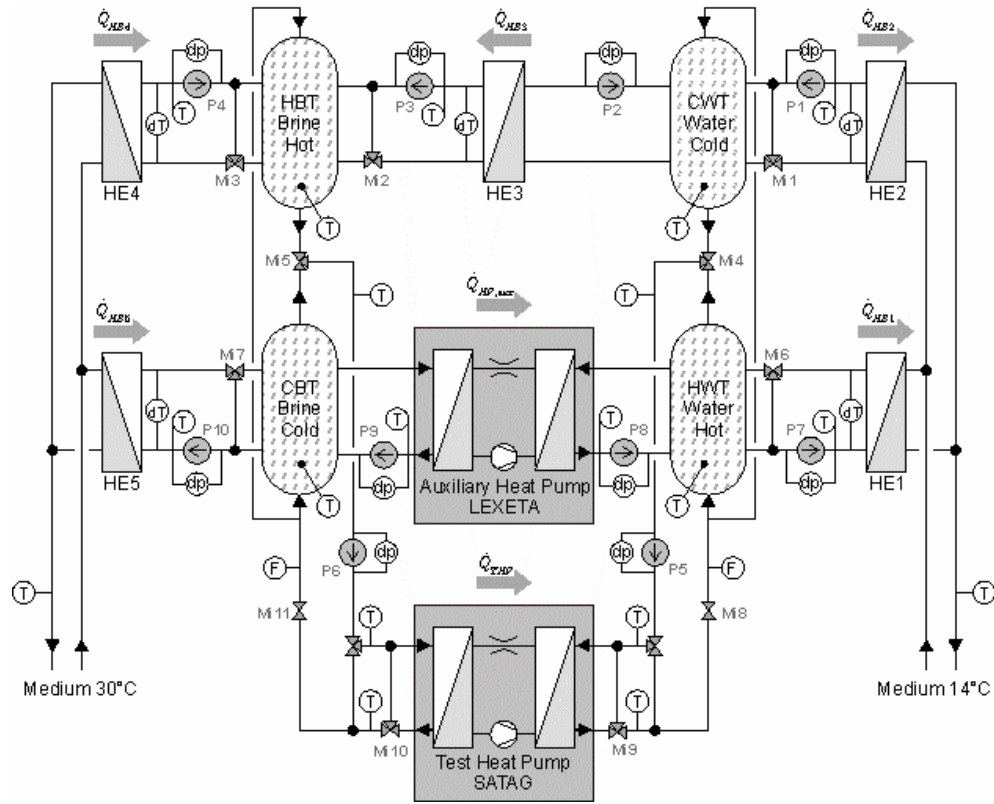
Fig. 2. Schematic diagram of the hydraulics of the test bench.
