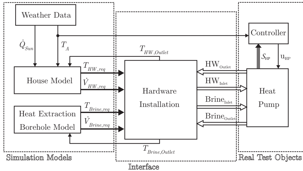
Fig. 1. Schematic representation of the test bench.
