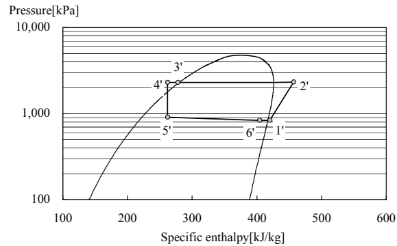
Fig. 7. P-H Diagram (the developing machine)
