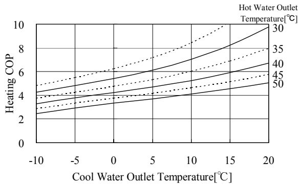
Fig. 11. Heating COP chart (developing machine) Fig. 12. Cooling COP chart (developing machine)
