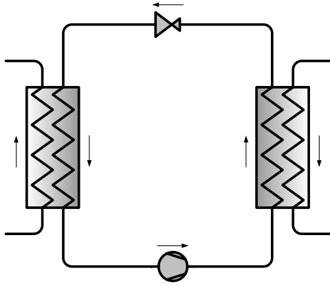
Fig. 4. Single-stage cycle
