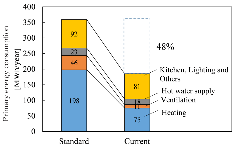
Figure 7. Estimated levels of reduced primary energy consumption
