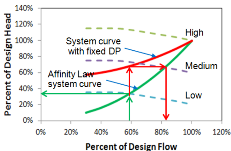
Figure 3. Conventional pumping control with fixed differential pressure set point results in overflow at part load conditions
