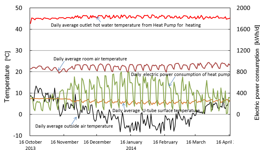
Figure 4. Annual performance of GSHP heating system of the primary school in Kuromatsunai town (16 th October, 2013- 16 th April, 2014)
