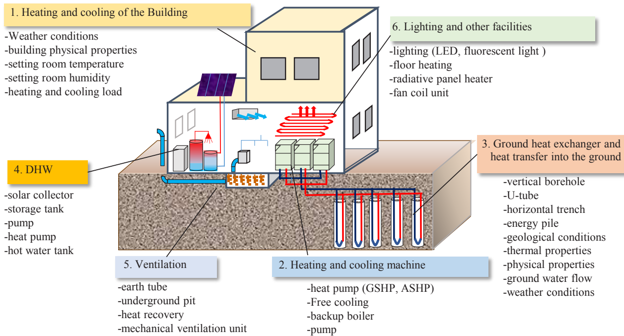
Figure 6. Structure of the ZEB simulator
