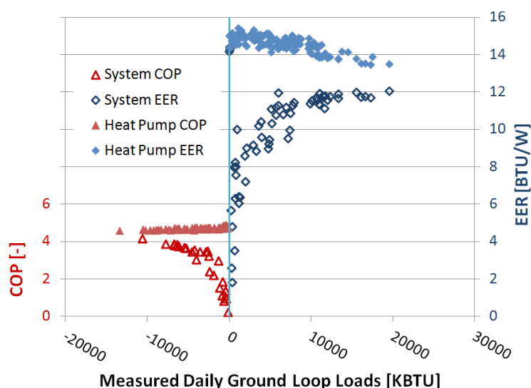
Figure 2. GSHP system efficiency vs. heat pump efficiency at various loading conditions (example results of case # 2)
