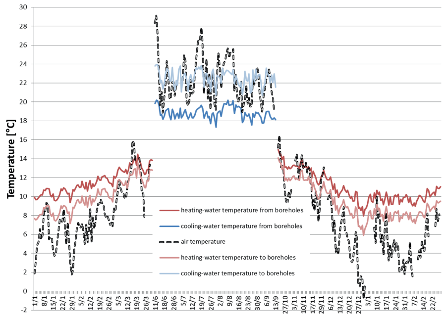
Figure 3. Daily average temperature of external air and of water from boreholes
