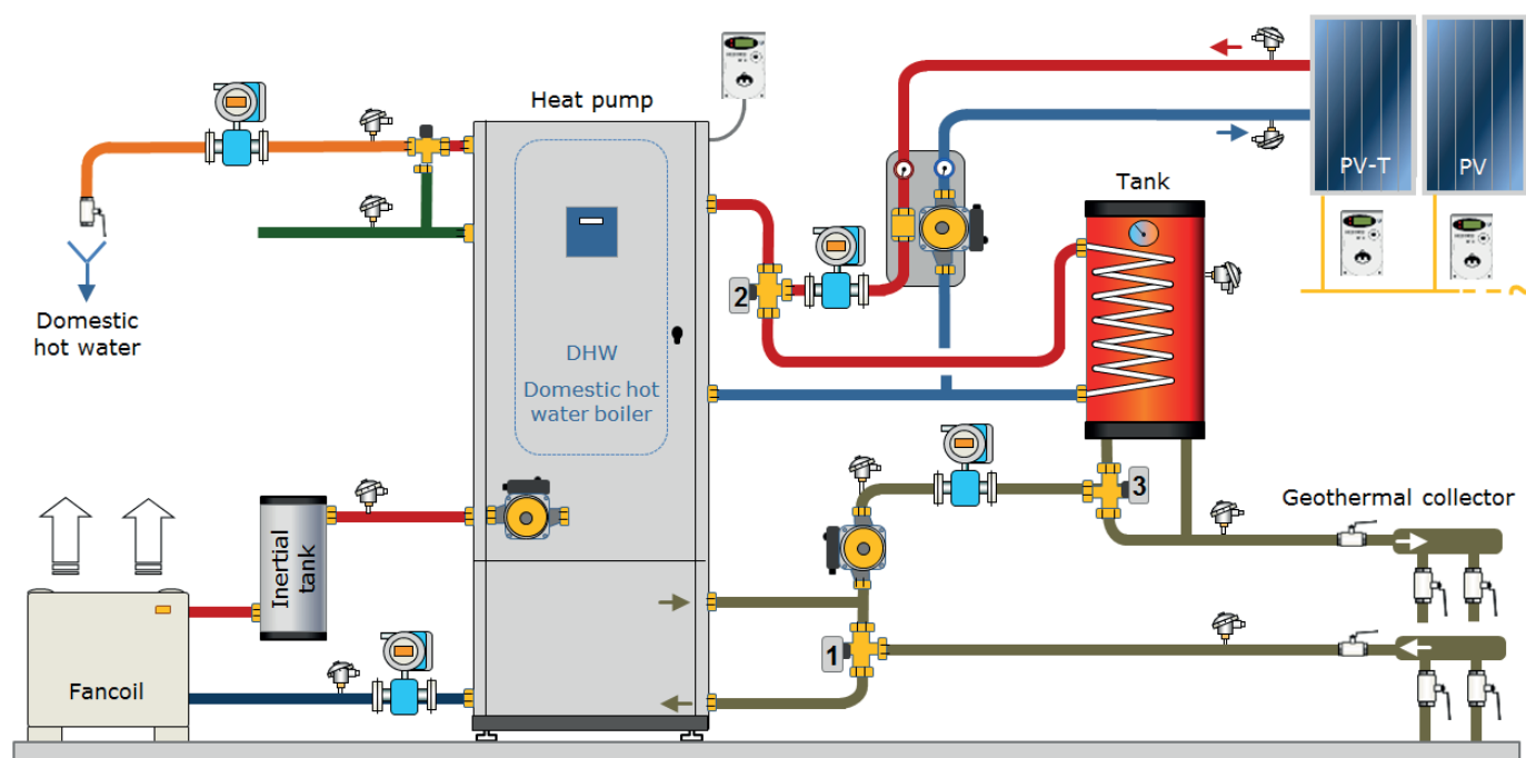
Figure 2. Plant scheme and monitoring system
