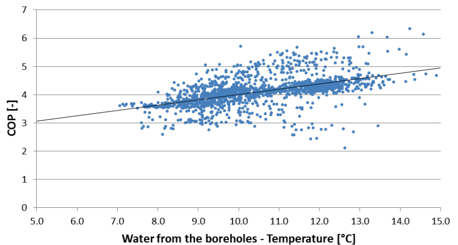
Figure 4. Hourly average COP related to hourly average water temperature from boreholes
