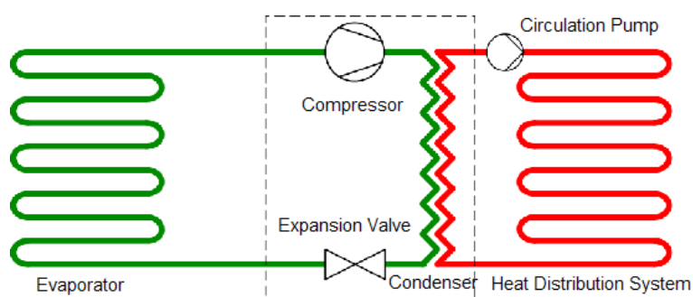
Figure 3. Direct Exchange Ground Coupled System
