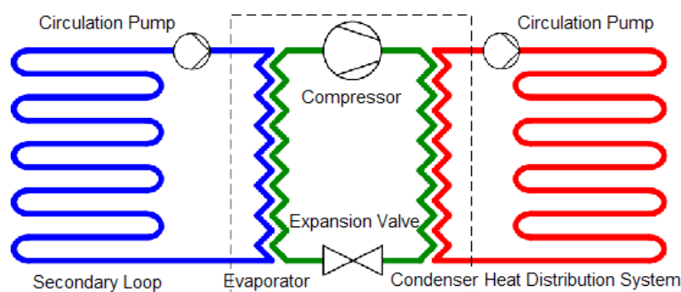
Figure 2. Secondary Loop Ground-Coupled System
