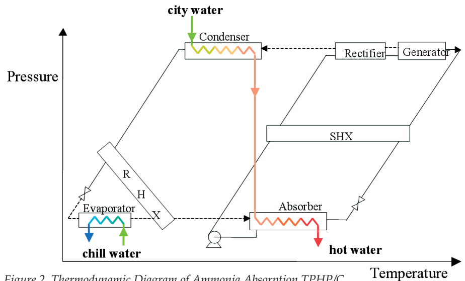
Figure 2. Thermodynamic Diagram of Ammonia Absorption TPHP/C
