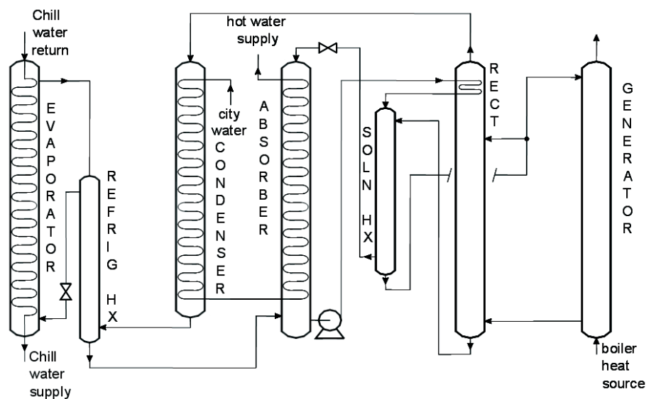
Figure 3. TPHP/C Flowsheet
