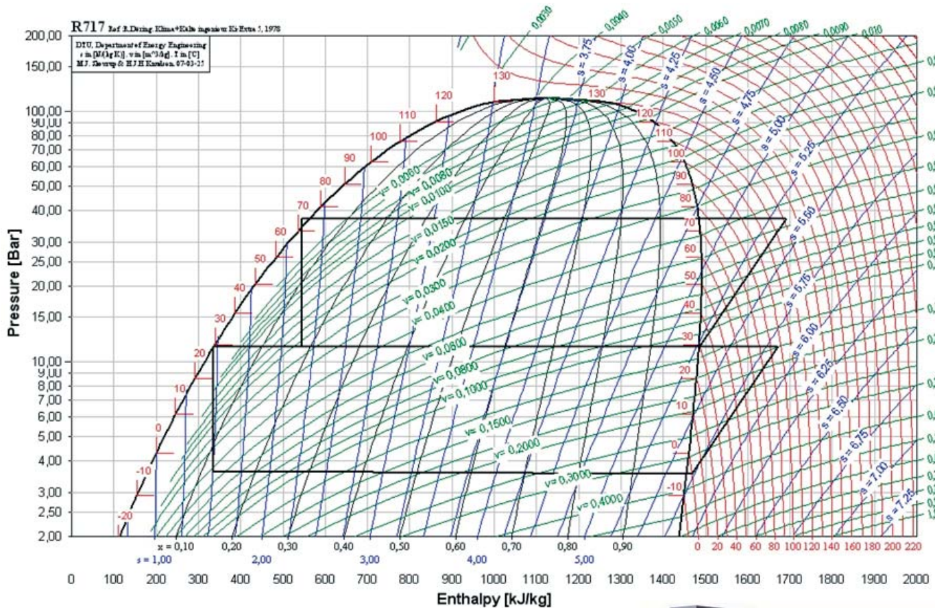
Example of an energy-efficient two-stage ammonia heat pump cycle at -5\text{ }^{\circ}\text{C} and 75\text{ }^{\circ}\text{C} evaporation and condensing temperatures. The isentropic compressor efficiency is 0.75 [5].
