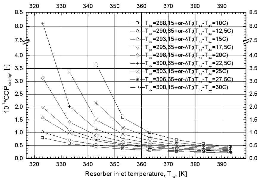
Figure 3. NH_3/H_2O coabsorbent hybrid heat pump COP vs. resorber maximum temperature T_{ra} . Modelling conditions: adiabatical single-stage vapor compression; mechanical efficiency = 0.9; resorber maximum temperature: T_{ra} = (323.15 \text{ to } 393.15) - \text{or } + \Delta T , where \Delta T = 0 to 10 \text{ } ^\circ\text{C} ; absorber minimum temperature: T_{de} = 278.15 + \text{or } - ; mixer concentration: y_{mix} = 0.7 ; absorber outlet concentration: y_{mix} + 0.05
