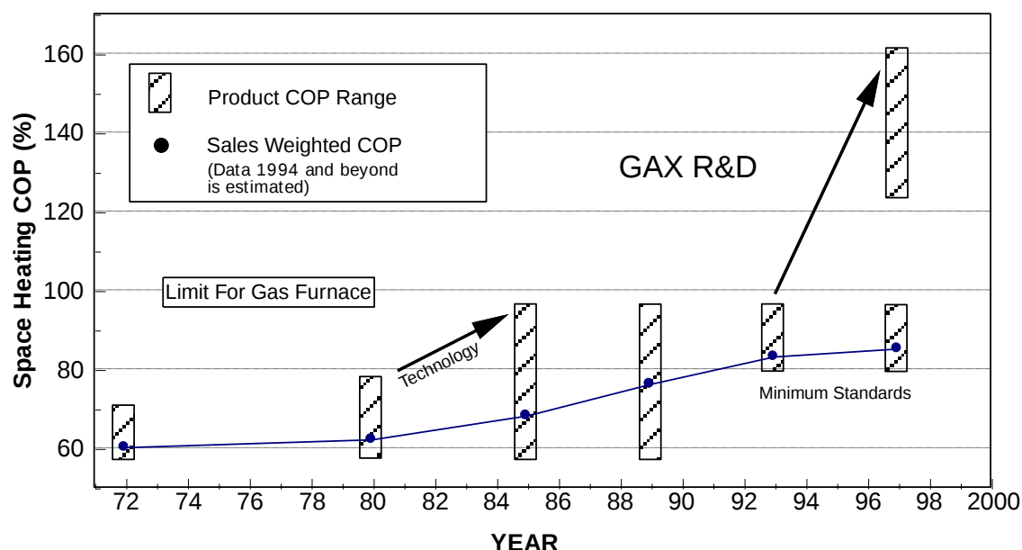
Figure 1. Comparison of Heating Efficiency of Gas Furnace and GAX Heat Pump.
