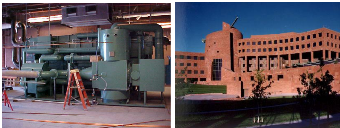
Figure 5. Triple-Effect, Direct-Fired Absorption Chiller Installed at the Clark County Government Center, Clark County, Nevada.
