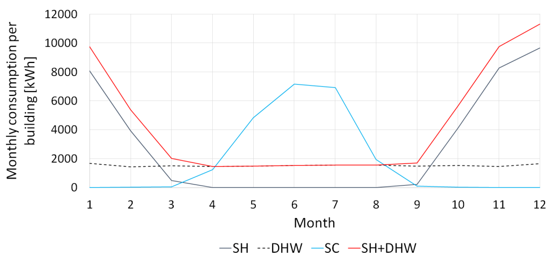
Fig. 1: Typical monthly consumption profiles for a single building of 500 m 2 . The different curves correspond to space heating (SH), domestic hot water (DHW), total heating (SH+DHW) and space cooling (SC).
