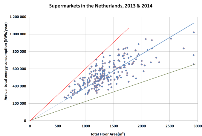
Figure 3. The distribution of the total energy consumption of a collection of supermarkets from the Netherlands shows that the total annual energy consumption can vary considerably for supermarkets of the same size. The red line denotes the least efficient supermarket (56 % above average energy consumption), the green line denotes the most efficient supermarket (42 % below average energy consumption).
