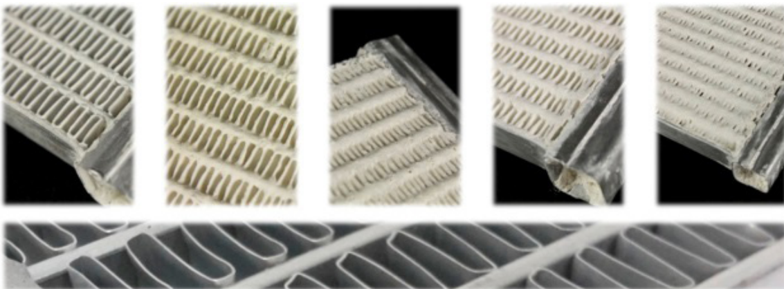
Figure 1. Coated adsorber heat exchangers for adsorption heat pumps. Binder-based coatings allow a flexible use of various adsorbents. Due to enhanced heat and mass transfer, both power density and COP can be increased significantly compared to adsorbents with adsorbent pellet beds.
