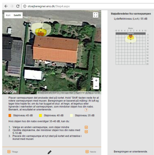
Figure 3. Visualization of the sound power level of a heat pump using the “Heat Pump Sound Emission Calculator” of the Danish Energy Agency.
