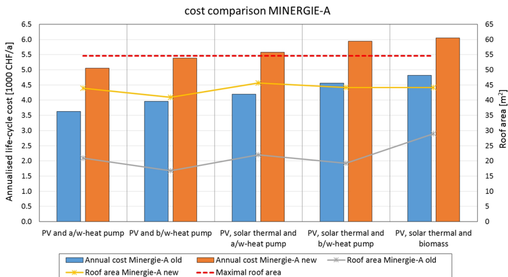
Figure 2. Comparison of old and new Net Zero Energy Building requirements according to the Minergie-A label regarding annualised system cost of different heat generation systems.
