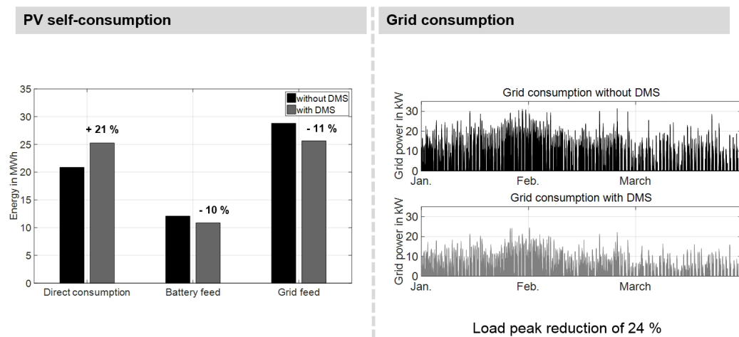
Figure 1. Simulation results of load management of heat pump and storage for grid supportive operation in the project HerzoBase of TH Nuremberg.
