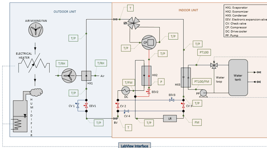
Figure 2. Modelling domestic hot water systems
