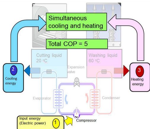
Figure 2. Application of heat pumps to cutting and washing processes.
