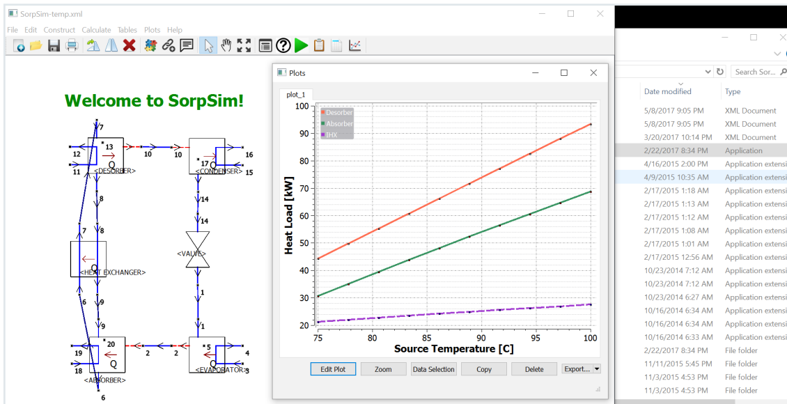
Figure 2. Screenshot of Sorption system Simulation program (SorpSim) developed by ORNL and Purdue University for flexible steady-state simulation and analysis of a wide range of sorption cycles with user-friendly features and parametric analysis functions. The isotherm database SorpPropLib, developed with input from Annex 43 participants, will be dynamically linked as an external library to SorpSim, supporting simulation and isotherm inquiry function in the SorpSim Graphical User Interface (GUI).
