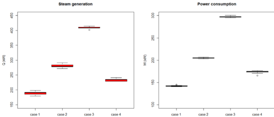
Figure 8. Steam generation and power consumption for the four cases. The steam generation is calculated from the flow of feed water, the feed water temperature and steam pressure. The power consumption is for the main motor and is sampled from the variable frequency drive.
