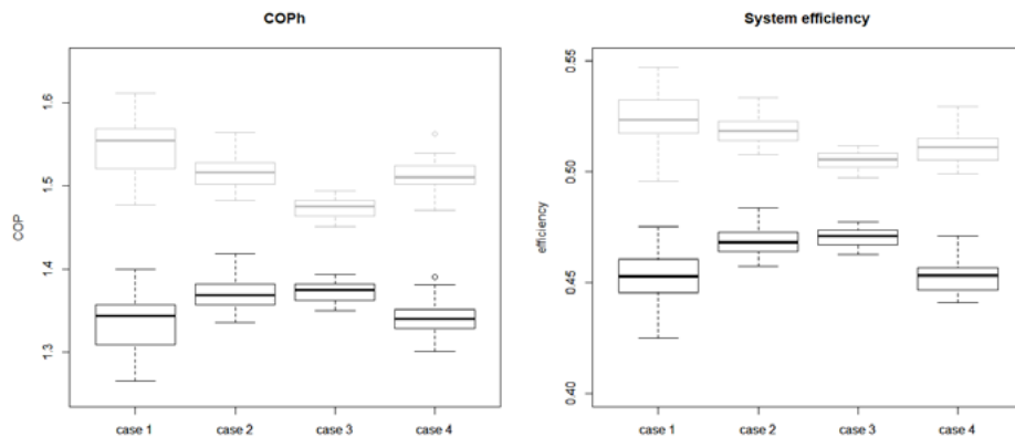
Figure 9. The coefficient of performance is defined as heat used to generated steam divided by the main motor consumption (i.e. COP_h = Q_h/W ). The system efficiency is defined as the measured COP_h divided by the Carnot COP (i.e. \eta_{system} = COP_h/COP_{carnot} ). The box and whisker plots in grey are estimated values for a fully thermally insulated heat pump.
