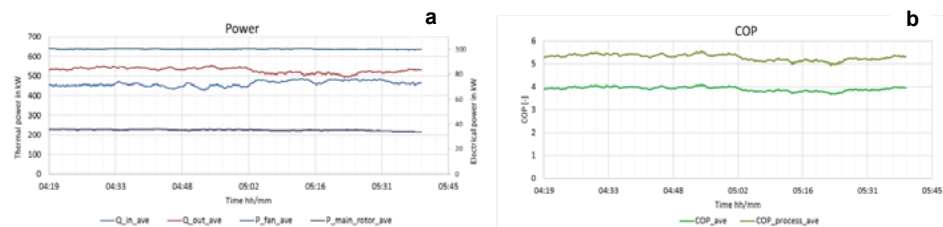
Figure 8: Thermal and electrical power (a), COP (b)
