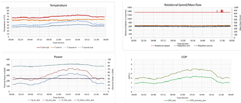
Figure 12: Test data, 3 rd day
