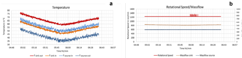
Figure 5: Temperature of sink and source (a), mass flow and rotational speed (b)
