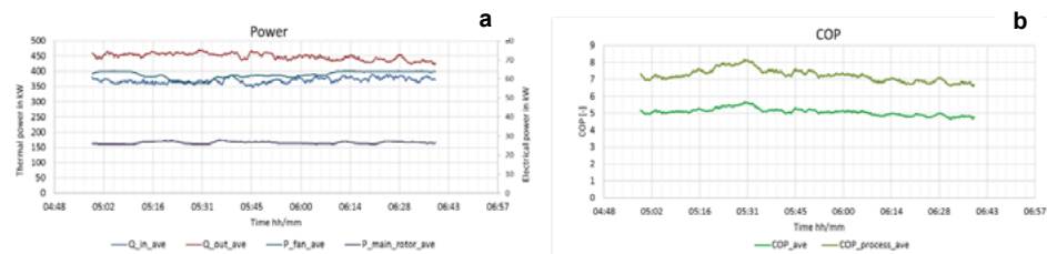
Figure 6: Thermal and electrical power (a), COP (b)
