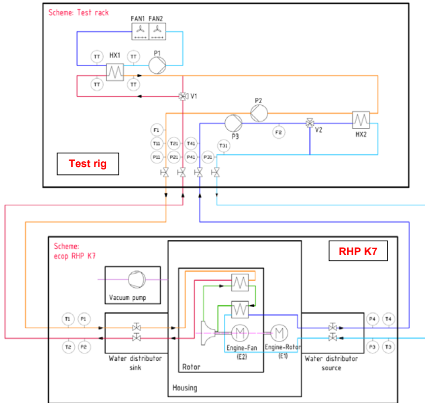
Figure 4: Simplified scheme of the test rig and RHP-K7
