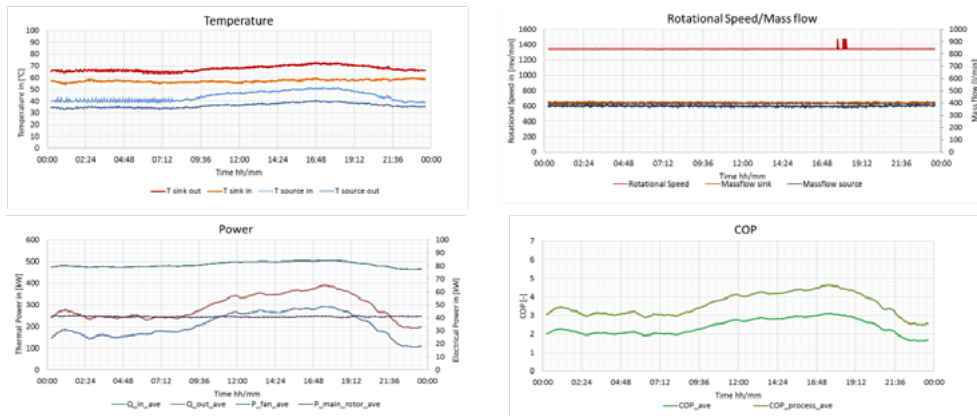
Figure 11: Test data, 2 nd day
