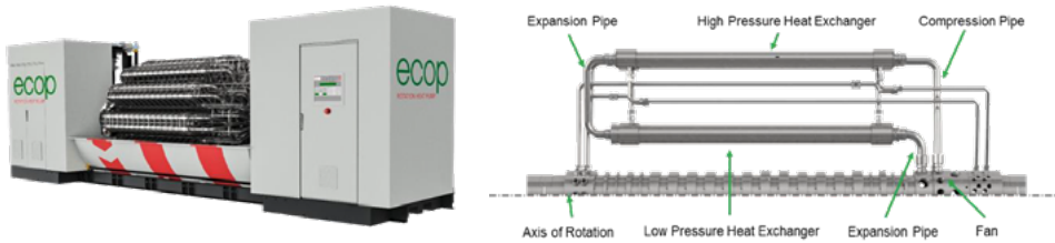
Figure 1: Design of a Rotation Heat Pump
