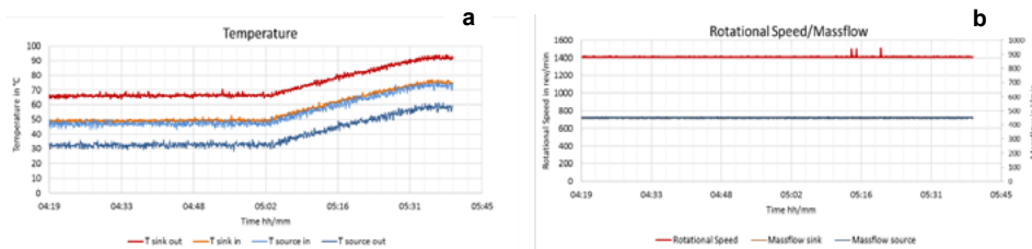
Figure 7: Temperature of sink and source (a), mass flow and rotational speed (b)
