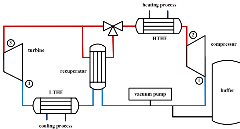
Figure 3: Simplified piping and instrumentation diagram of the Brayton cycle heat pump of the DLR Institute of Low-Carbon Industrial Processes in Cottbus (Germany)
