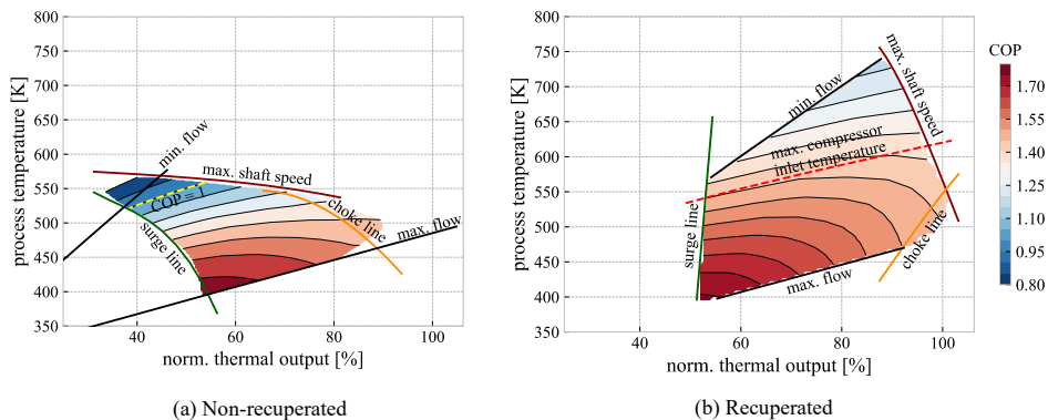
Figure 6: Operating envelopes with COP
