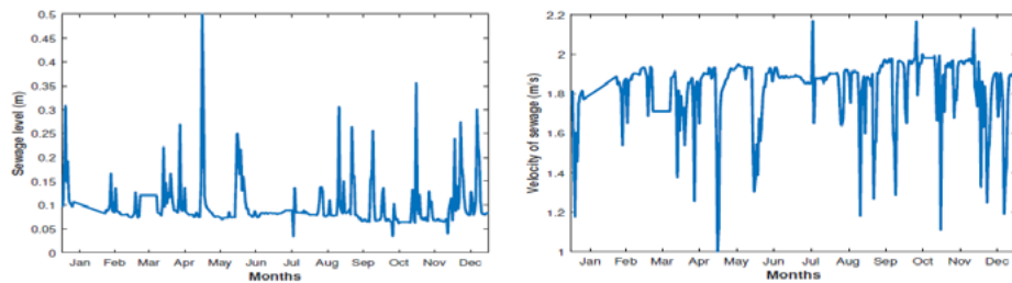
Fig. 3. Daily averaged sewage level (left) and velocity (right) of the sewage flow in 2018.
