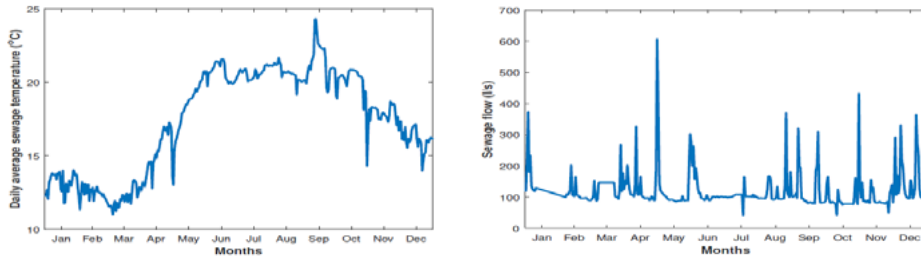
Fig. 2. Daily averaged temperature (left) and volumetric flow rate (right) of the sewage flow in 2018.
