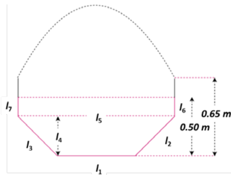
Fig. 1. Schematic of the cross section of the sewage channel.
