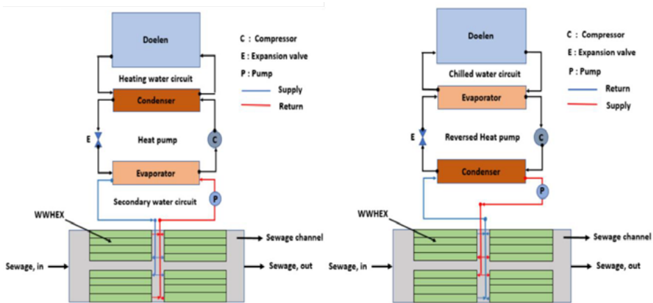
Fig. 4. WWSHP system as connected during the winter season (left) and summer season (right).
