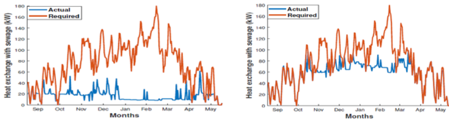
Fig. 7. Difference between the required (red) and recovered (blue) heat from the sewage for the 29 mm tube. Left for tubes of 12 m; right for tubes with 30 m.
