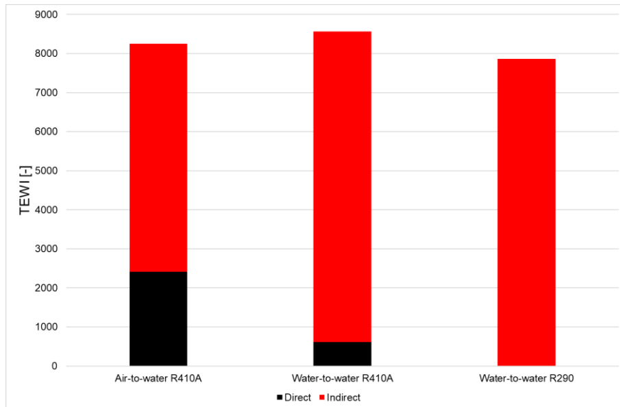
Fig. 3. TEWI of the three systems.
