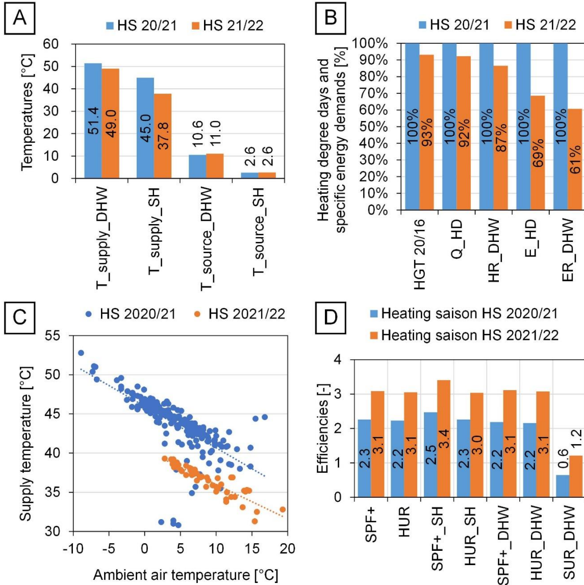
Fig. 2. Comparison of two heating seasons, HS 2020/21 and HS 2021/22, in a renovated single-family house from 1975 (Object No. 24 equipped with an inverter-regulated AWP [9]) after control optimization on the HP. (A) Change of the supply and source temperatures in heating and DHW mode, (B) Comparison of the heating degree days and the specific thermal and electrical demands in heating and DHW mode (thermal demand decreased by 8 %, electrical demand decreased by 31 %), (C) Adjusted heating curve in HS 2021/22 (approx. 7 K lower supply temperature) compared to HS 2020/21 after a reduction of the temperature rise in the buffer tank, (D) Comparison of the efficiencies in heating, DHW, and combined operating modes for the heating seasons HS 2020/21 and HS 2021/22 (Data source: [9]).
