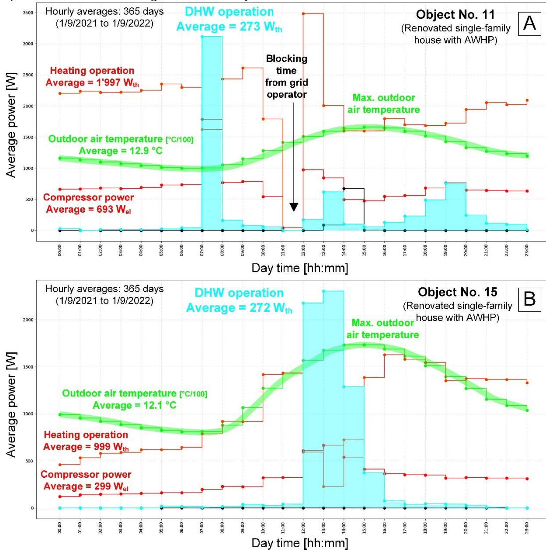
Fig. 3. (A) DHW operation at Object No. 11 occurs predominantly between 7:00 and 8:00 when the outdoor air temperature is low. The highest outdoor air temperatures are measured between 15:00 and 16:00. Between 11:00 and 12:00, blocking times of the electrical grid operator are active. (B) DHW operation at Object No. 15 is shifted to high outdoor air temperatures between 12:00 to 16:00. The operating window could even be moved to 14:00 to 17:00 to profit from the highest outdoor air temperature of 17.2 °C.
