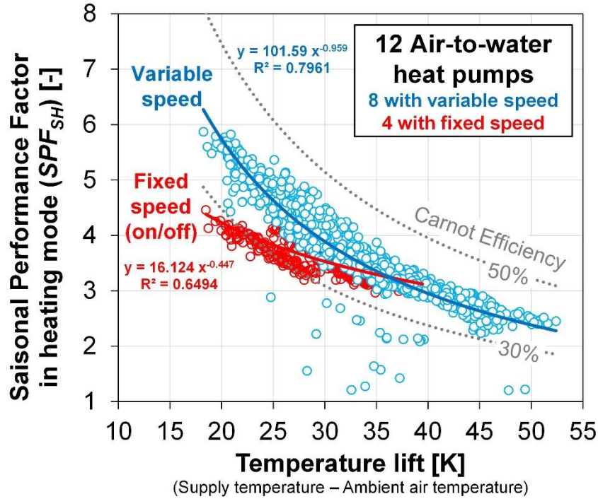
Fig. 4. Comparison of the seasonal performance factor of variable speed and fixed speed (on/off) AWHPs in heating mode as a function of the temperature lift between supply temperature and ambient air temperature as the heat source (ranging from 0 to 10 °C). Each point is a daily average (Data source: [8], [9]).
