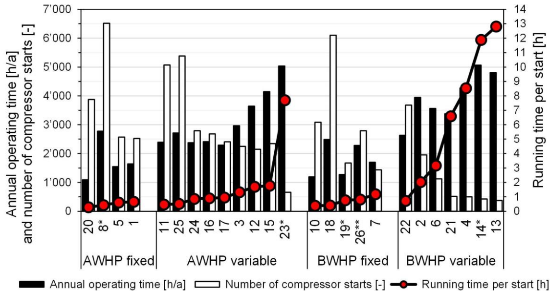
Fig. 5. Annual operating time, number of compressor starts, and running time per start of different fixed speed and variable speed AWHPs and BWHPs in HS 2021/2022, *Objects with separate DHWHP. **2 HPs with 4 parallel compressors (Data source: [9]).
