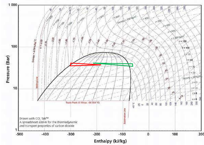
Figure 3. Illustration of Possible CO 2 State Points (Green → Chiller-to-Receiver Loop; Red → Receiver-to-AHU Loop)
