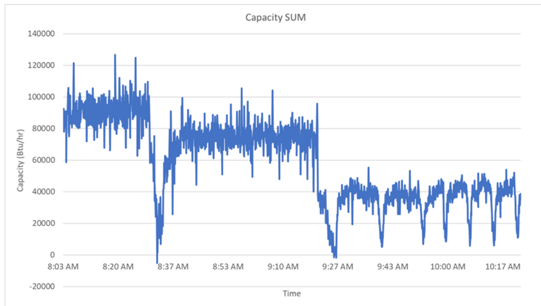
Figure 4. Cooling capacity vs time (low ambient test)
