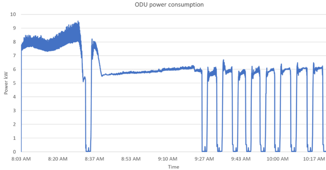
Figure 5. Chiller power vs. time (low ambient test)
