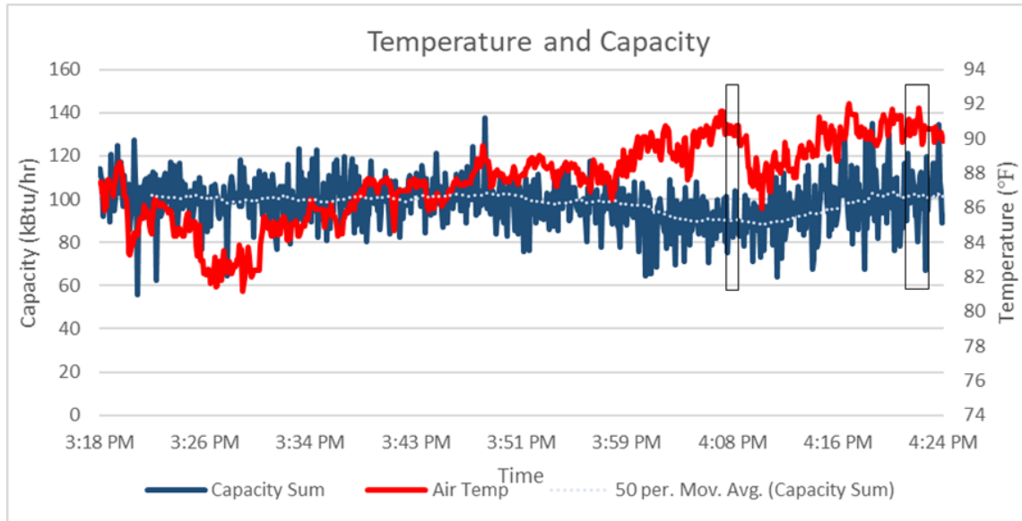
Figure 6. Cooling capacity and outdoor temperature versus time (high ambient test)
