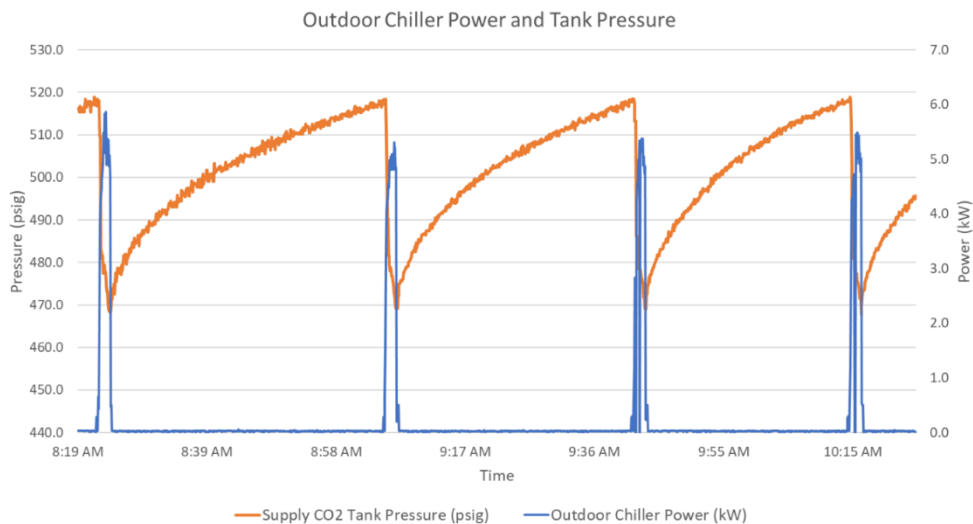
Figure 4. Outdoor chiller and tank pressure versus time (standby operation test)
