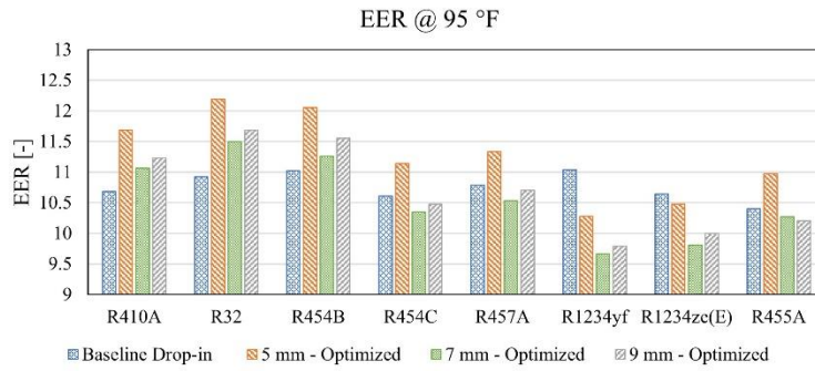
Fig. 8 shows the cooling performance comparison at 95 °F. For R410A, R32, R454B, R455A and R457A, the optimized 5-mm tube heat exchangers yield 9.4%, 11.6%, 9.4%, 5.5% and 5.1% EER improvements, respectively. Except R32 and R454B, using 7-mm tube and 9-mm tube with GWP less than 150 refrigerants yields performance degradation compared with the baseline drop-in test. For refrigerants with GWP less than 150, the optimized systems have the capacity to improve system performance. In this study,
