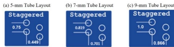
Fig. 5. Horizontal spacing and vertical spacing in inch for (a) 5-mm tube HX; (b) 7-mm tube HX; (c) 9-mm tube HX.
