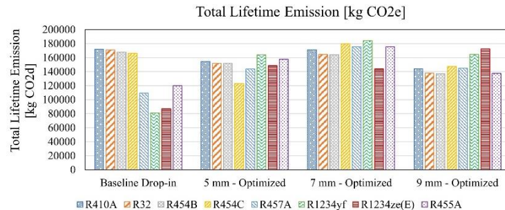
Fig. 16. Total greenhouse gas emissions of the baseline and low-GWP optimized systems.
