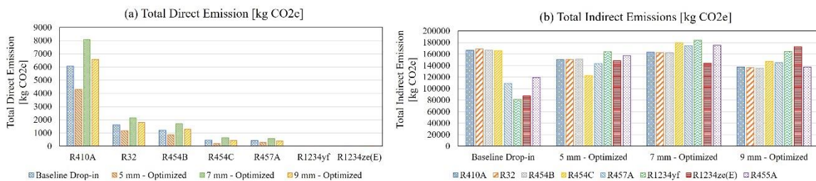
Fig.15. Greenhouse gas emissions of the baseline and low-GWP optimized systems (a) Direct Emission; (b) Indirect Emission.
