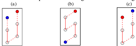
Fig. 2. Heat exchanger circuitry patterns: (a) counterflow, (b) mixed flow, (c) parallel flow
