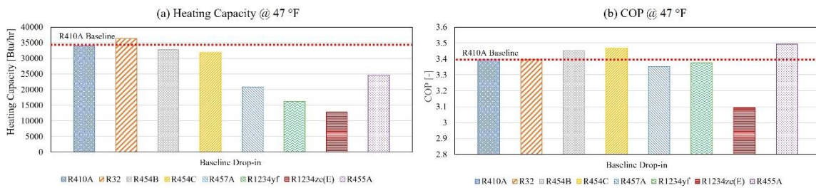
Fig. 7. Baseline System Drop-in Heating Performance at 47 °F (a) Heating Capacity; (b) COP
