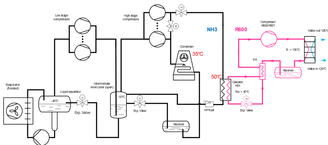
Figure 5: Add-on HP for steam generation on top of an existing NH 3 Industrial refrigeration system
