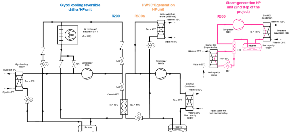
Figure 4: Combination of hydrocarbon one-stage systems for cooling and process heating in a Dutch brewery (Rangelov and Kerkhof, 2025)
