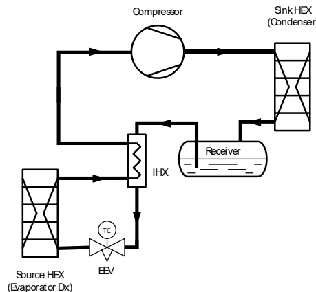
Figure 2: One-stage system
