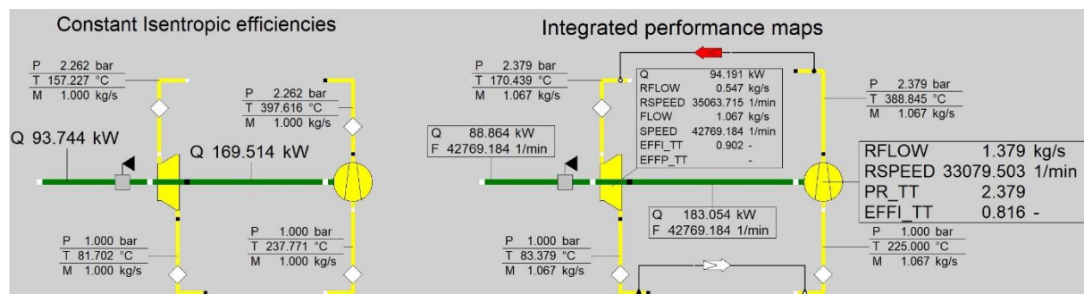
Figure 5: Turbo-unit development
