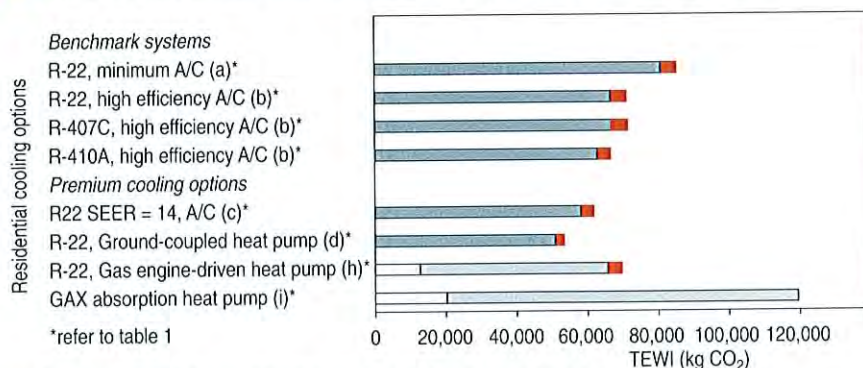
▲ Figure 3: TEWI for residential cooling options, Florida, USA.
