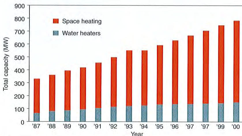
▲ Figure 2: Total installed capacity in Austria, 1987-2000
