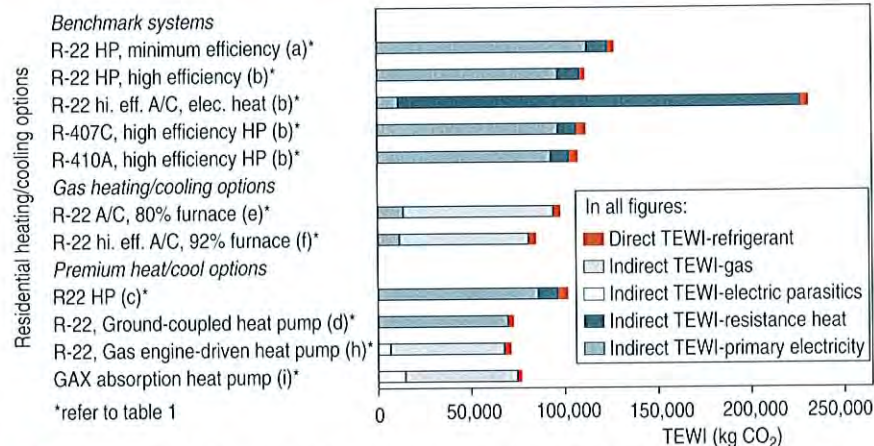
▲ Figure 1: TEWI for residential heating/cooling options, Pittsburgh, Pennsylvania, USA.
