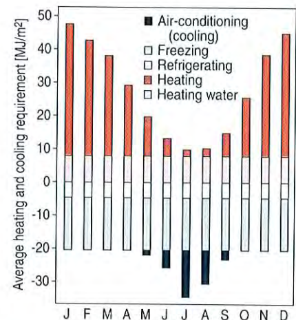
▲ Figure 1: Measured average monthly values for heating and cooling in a restaurant
