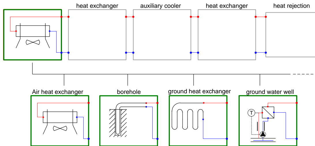
Fig. 4-20: Heat sources for heat pump operation: Air-heat exchanger, boreholes geothermal collectors (ground heat exchanger) or ground water well,
