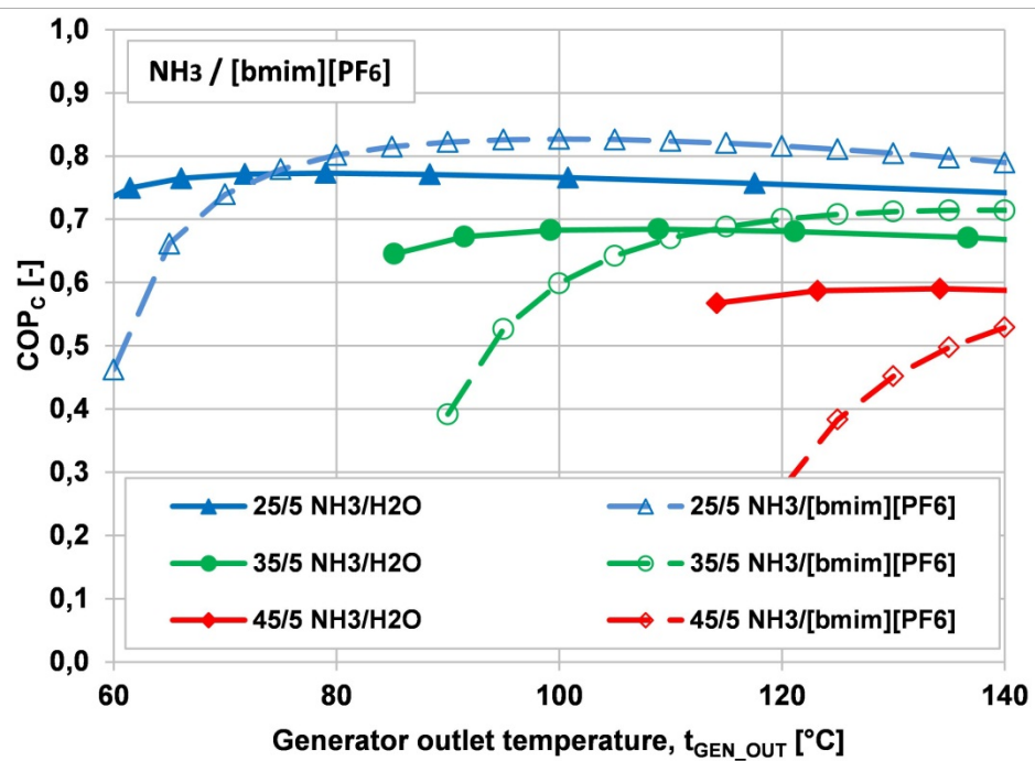
Fig. 3-22: Simulation results of the COP for t_{ABS}/t_{EVA}=25/5^\circ C , 35/5^\circ C and 45/5^\circ C of NH_3/[bmim][PF_6] AHP-processes without rectification column in comparison to a conventional NH_3/H_2O AHP-process with rectification column depending on the generator outlet temperature
