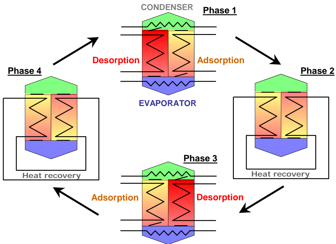
Fig. 1-4: Simple adsorption schematic with heat recovery phase
