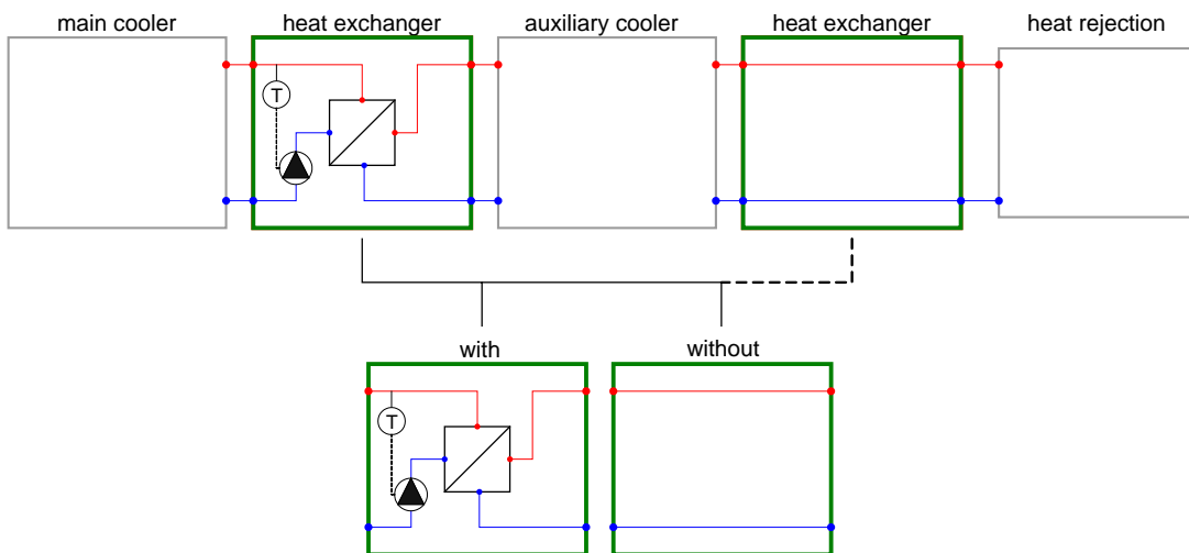
Fig. 4-14: Heat rejection sub-system: optional heat exchangers for separation of thermally driven chiller, auxiliary cooler and main cooler.
