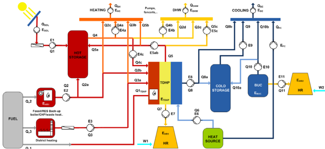
Fig. 4-2: Max system representation for a heating and cooling, direct and/or indirect fired application
