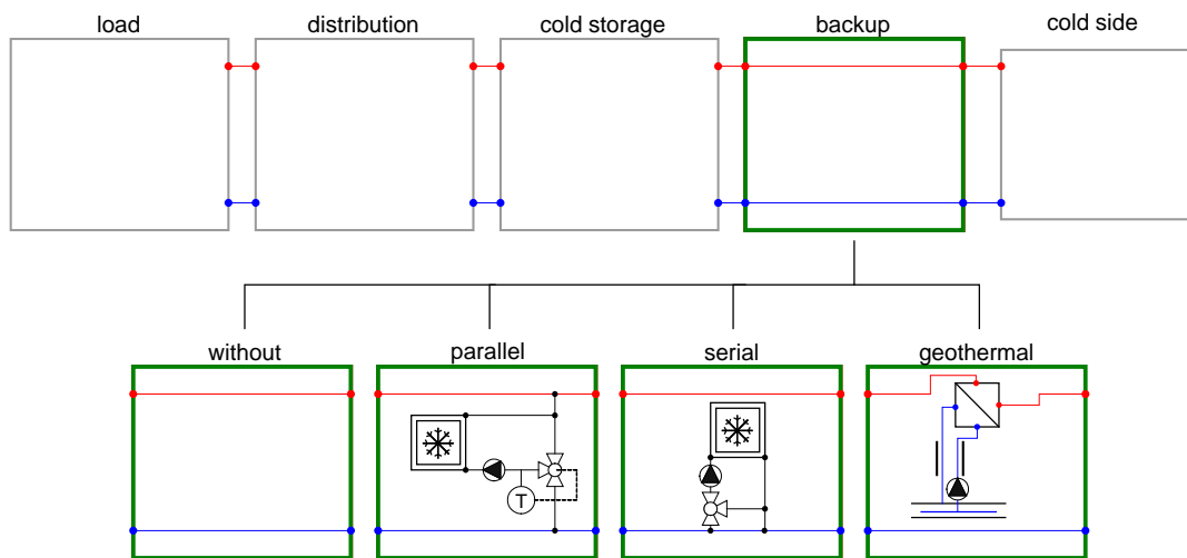
Fig. 4-19: Chilled water sub-system: Integration of a compression chiller or a ground water well as backup cooling source.
