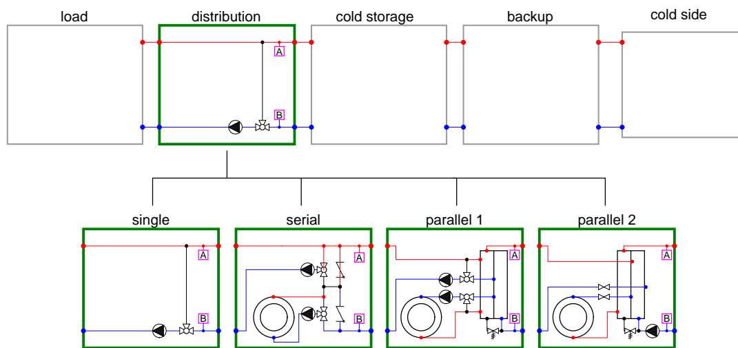
Fig. 4-17: Chilled water sub-system: Options for the distribution of the chilled water.
