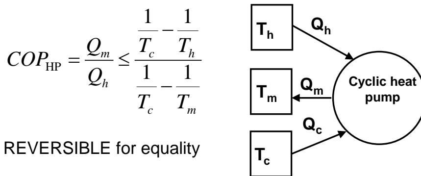
Fig. 1-2: Ideal thermodynamic limitations
