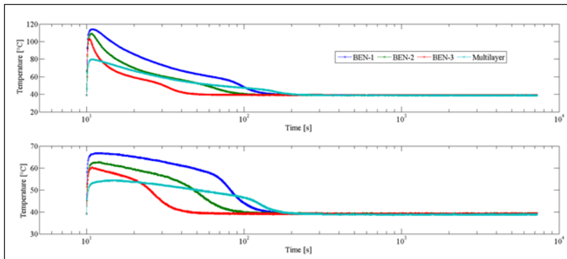
Fig. 3-8: Dynamic evolution of the surface temperature of the four tested samples: in the upper part after desorption against the vacuum pump, in the lower part after desorption against the condenser @ 30°C.
