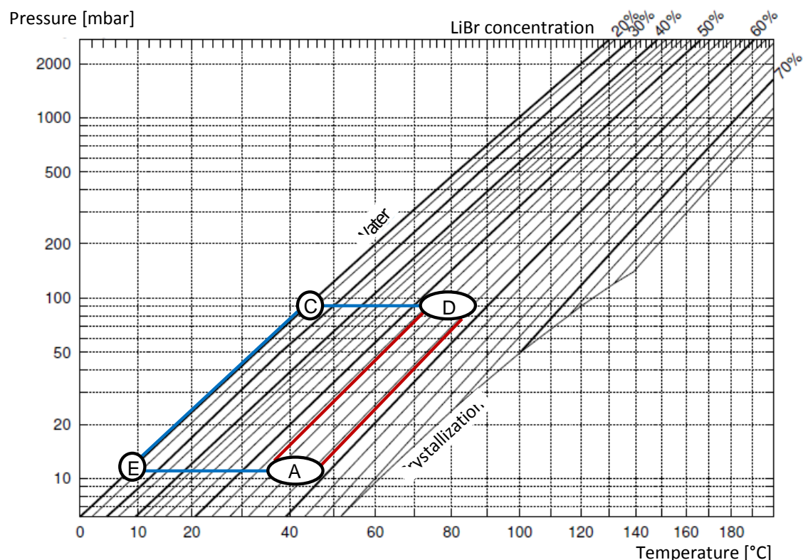
Fig. 1-16: Absorption heat pump cycle in the \ln p - 1/T -diagram of water/LiBr (Feuerecker 1994)
