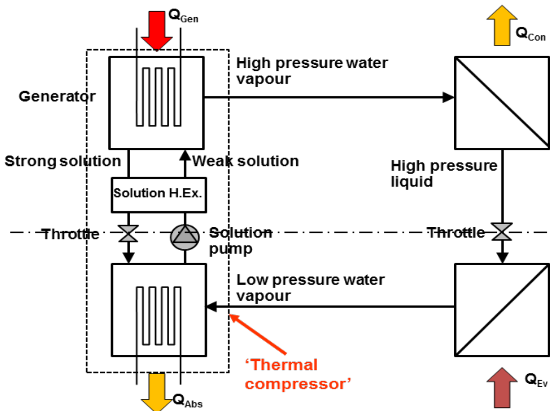
Fig. 1-3: Simple water - LiBr absorption cycle schematic
