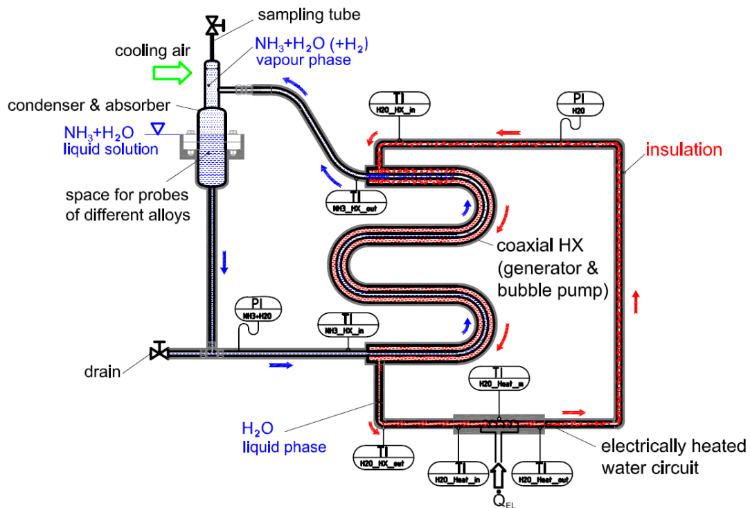
Fig. 3-23: Schematic drawing of the thermosiphon cycle test rig with indicated instrumentation
