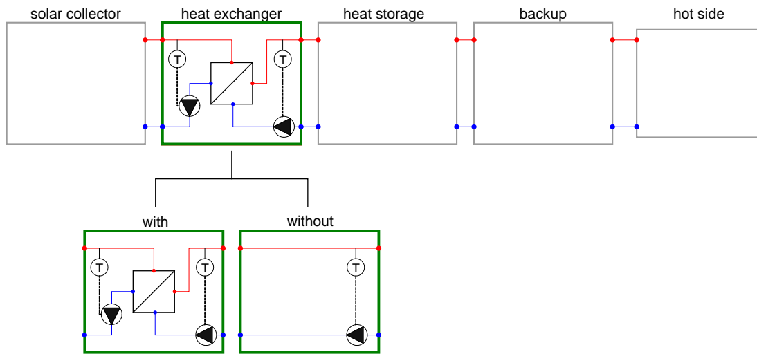
Fig. 4-8: Solar sub-system: heat exchanger for separation of primary and secondary solar loop.
