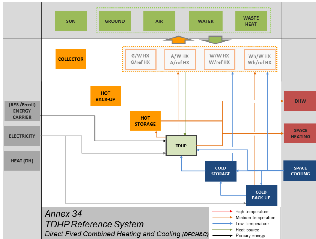
Fig. 2-4 Direct fired TDHP system for combined heating and cooling; “Square View” representation.
