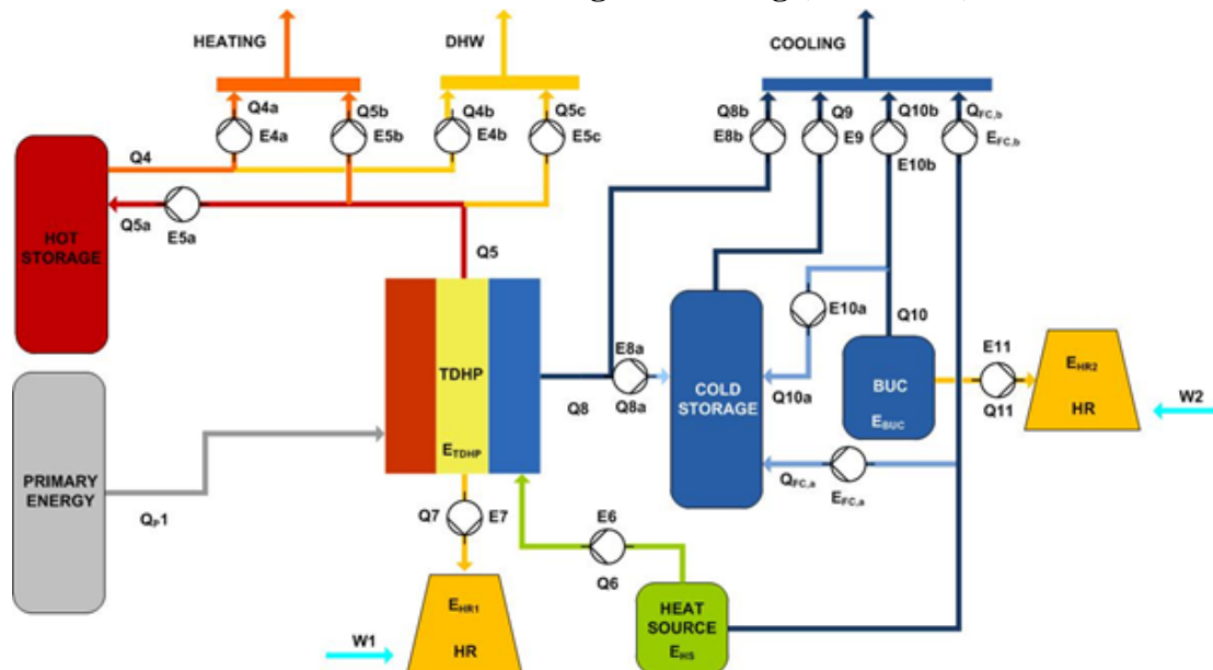
Fig. 2-3 Direct fired TDHP system for combined heating and cooling; modified SHC Task 38 representation.
