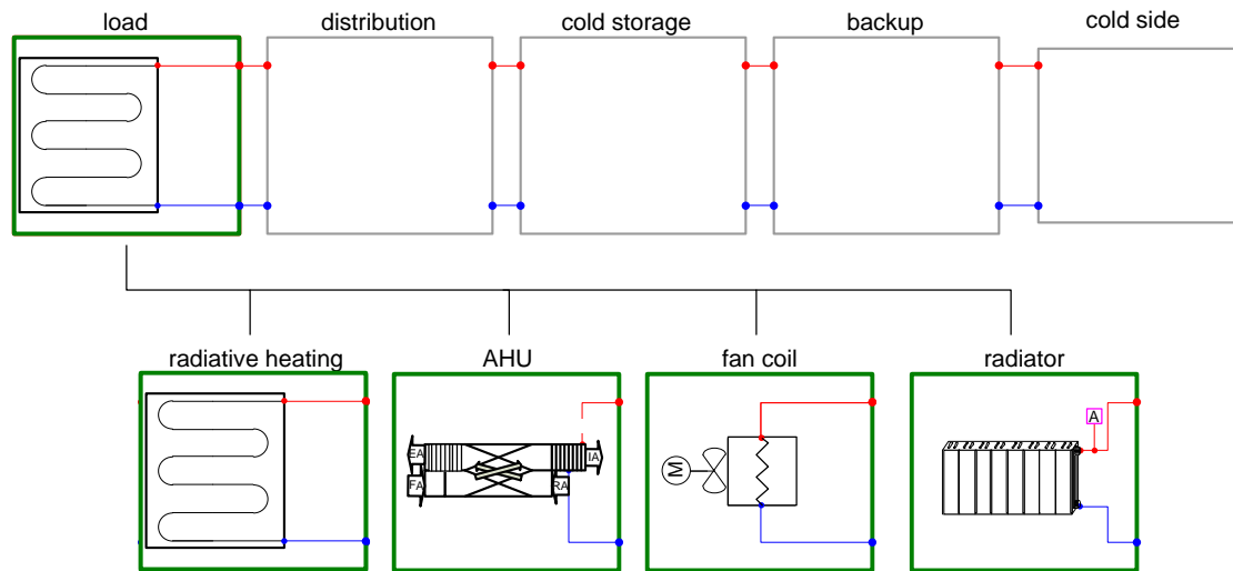
Fig. 4-15: Heating appliances for utilization of the heat output of the sorption heat pump at intermediate temperature level for space heating.
