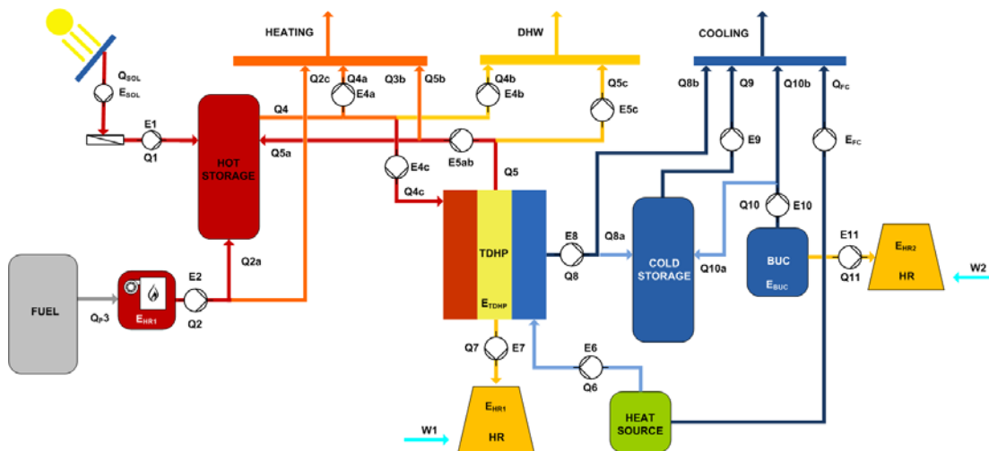
Fig. 4-3: Example of indirect fired heating and cooling application
