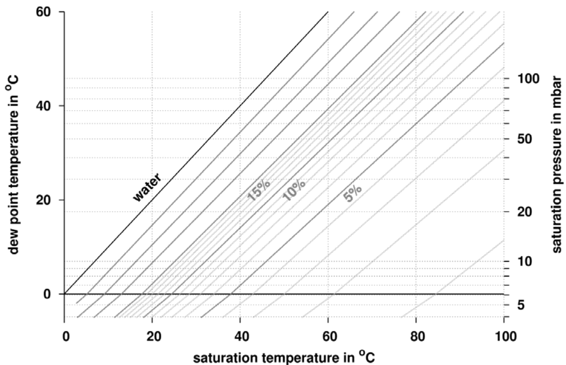
Fig. 1-18: Dühring-Diagram for Silica-Gel 127B. © Fraunhofer ISE
