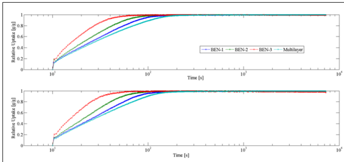
Fig. 3-7: Dynamic evolution of the relative uptake of the four tested samples: in the upper part after desorption against the vacuum pump, in the lower part after desorption against the condenser @ 30°C.
