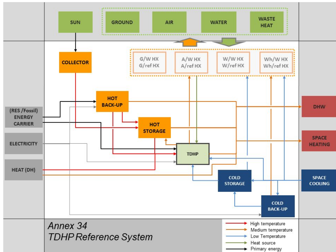
Fig. 2-2: Reference system for applications including TDHP: Modified SHC Task 38 representation (above), “Square View” (below).
