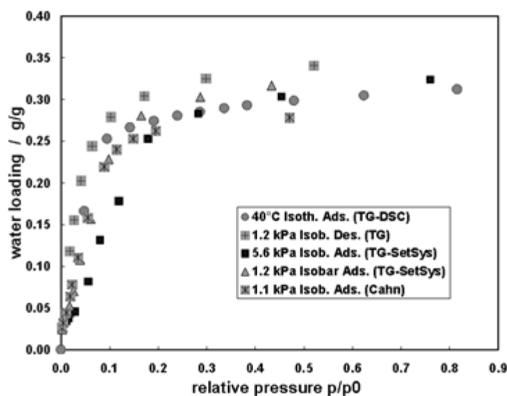
Fig. 3-16: Comparison of measurements for the SAPO-34 sample with different equipment and procedures.
