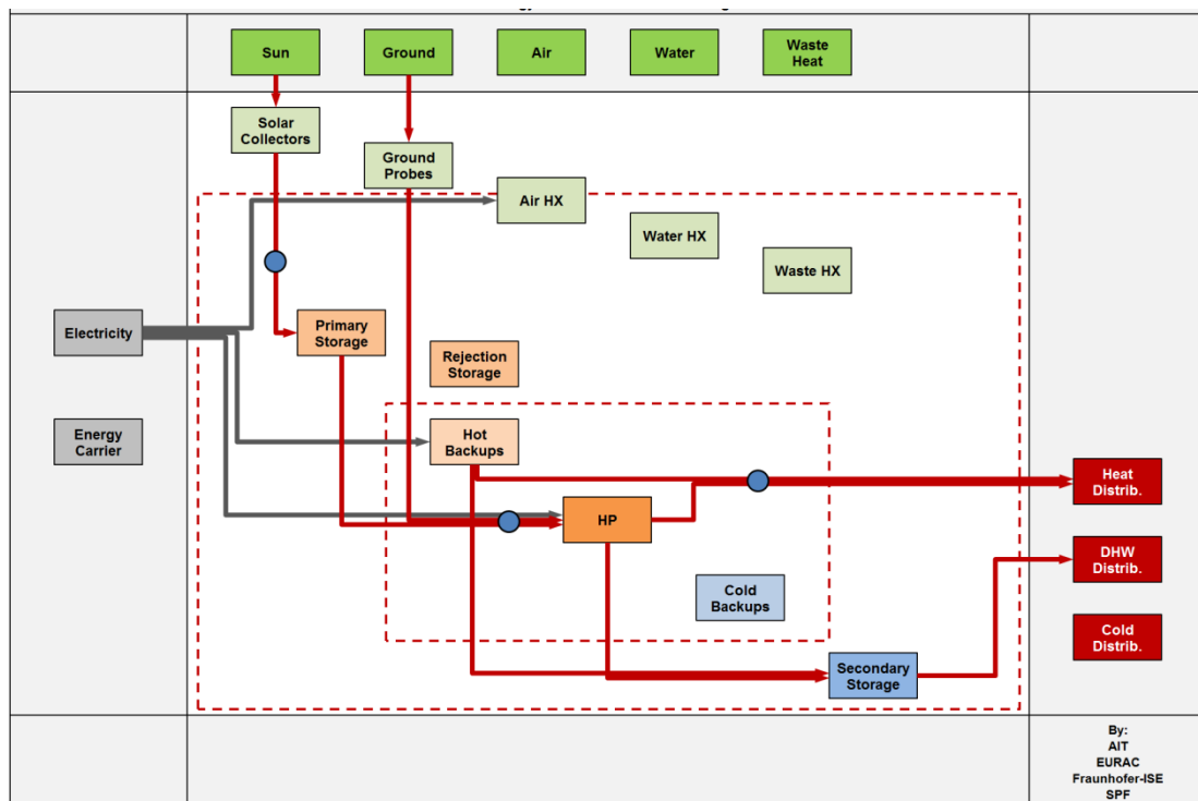
Fig. 4-24: Energy Flow Chart. Method with permission of IEA- SHC Task 44 -HPP Annex 38, 2011
