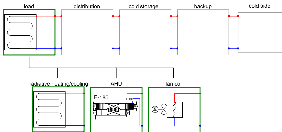
Fig. 4-16: Chilled water sub-system: Room-side installations for the transfer of the cooling effect.
