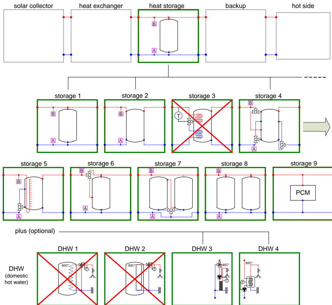
Fig. 4-9: Solar sub-system: options for the heat storage and domestic hot water preparation.
