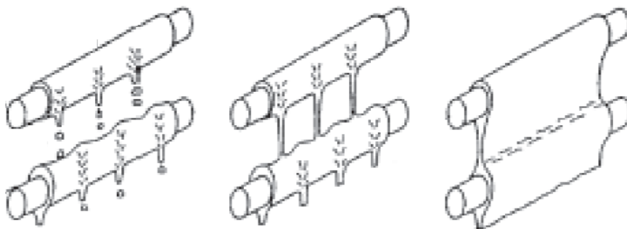
Fig. 1-7: Modes of falling films on horizontal tubes (Hu und Jacobi 1998, p. 323)(Hu 1998)
