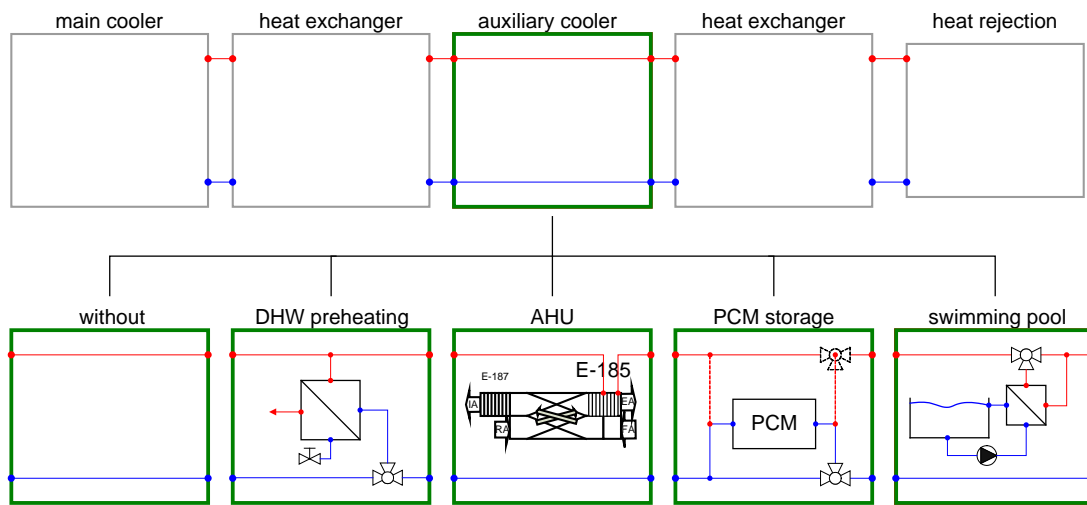
Fig. 4-13: Heat rejection sub-system: auxiliary coolers.
