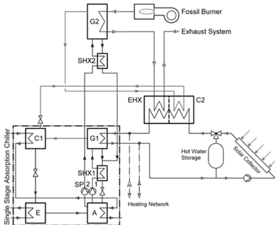
Fig. 1-15: Double-/Single-effect absorption solar thermal plant for flexible heating and cooling. (Riepl, Gurtner et al. 2011)
