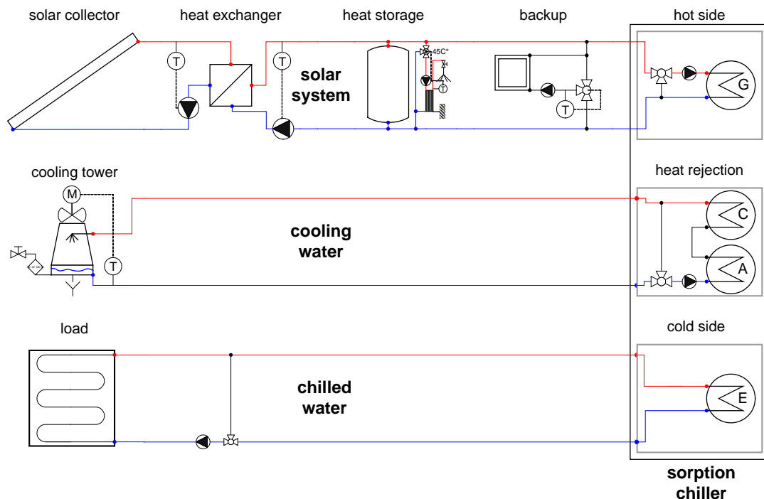
Fig. 4-4: Basic solar cooling system: Thermally driven chiller coupled to solar thermal system, cooling water loop, and chilled water loop.
