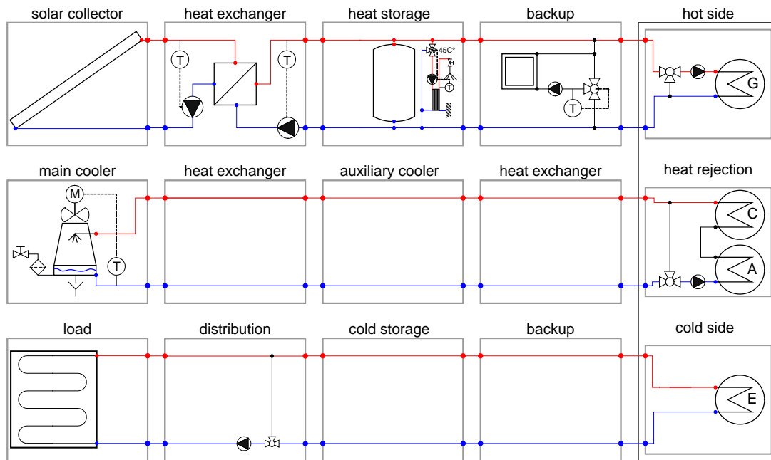
Fig. 4-5: Generic system: standardized system topology with placeholders for the integration of optional system components.
