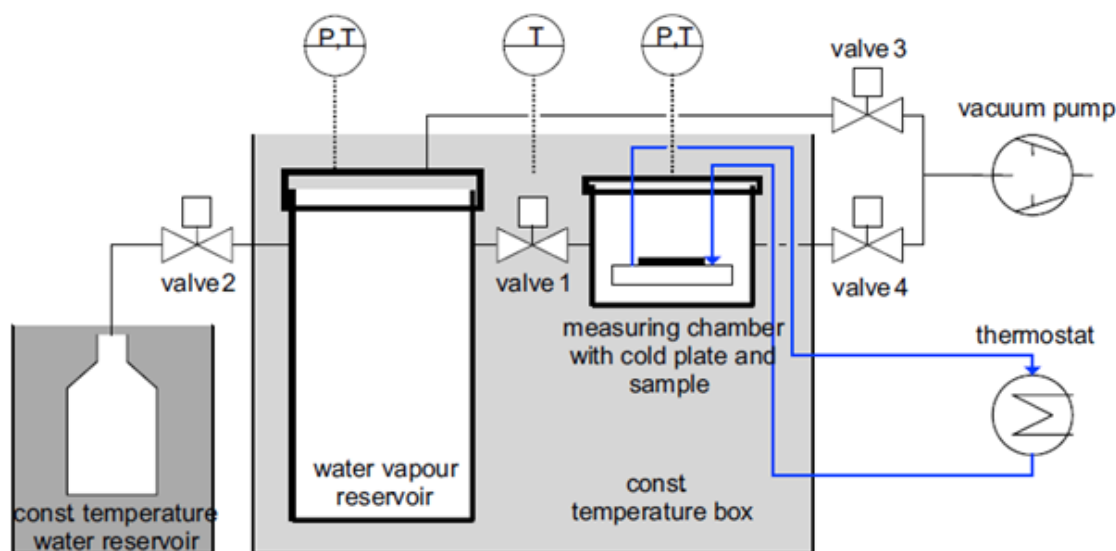
Fig. 3-4: Scheme of the entire kinetic measurement setup.
