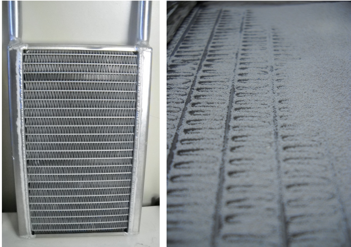
Fig. 1-9: Adsorbers developed at ITAE, Italy
