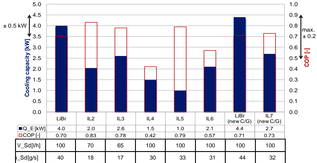
Fig. 3-20: Test results of water/LiBr and water/IL working pairs
