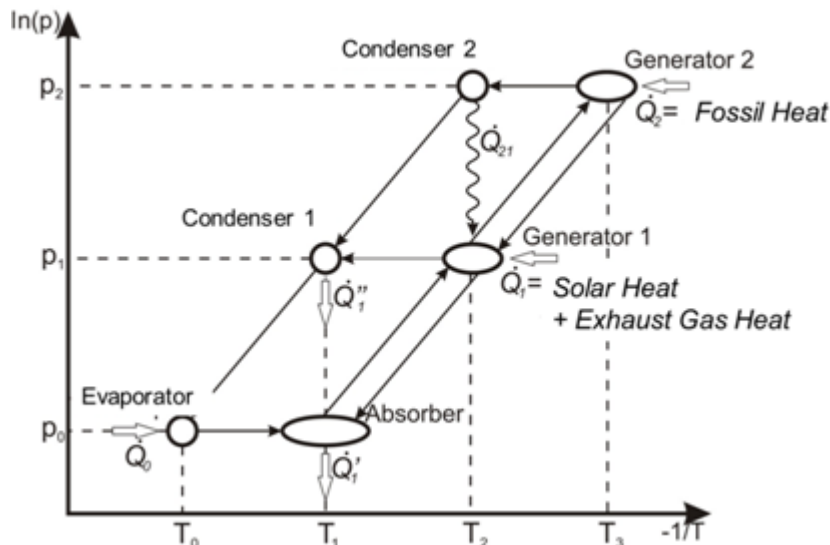
Fig. 1-14: Double-/Single-effect absorption cycle in the \ln p/-1/T -diagram (Riepl, Gurtner et al. 2011)
