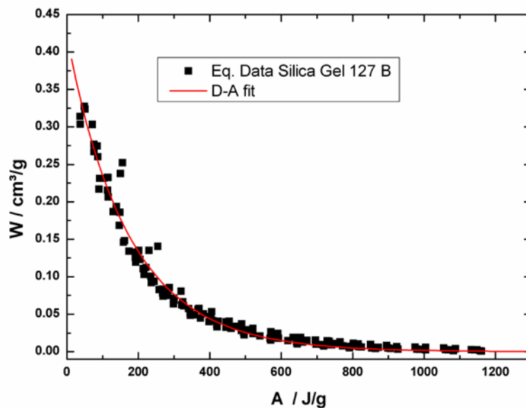
Fig. 3-17: Transformation according to D-A equation of the equilibrium points for water/Silica Gel.
