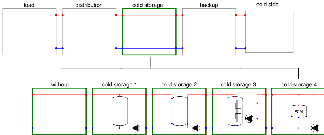
Fig. 4-18: Chilled water sub-system: Chilled water storage and latent cold storage (PCM, phase change material).
