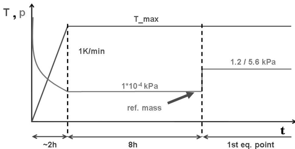
Fig. 3-12: Proposed measurement procedure, including sample pre-treatment and the first isobaric step.
