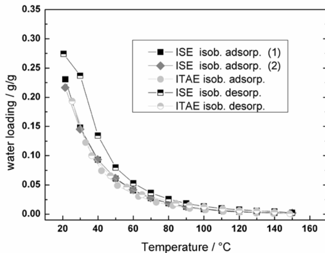
Fig. 3-13: Comparison of isobar adsorption measurements for Silica Gel 127 B at 1.2 kPa.
