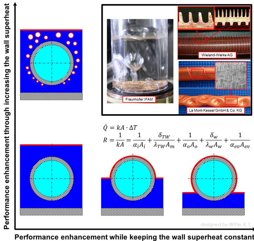
Fig. 3-10: Enhancement technics to increase the outer heat transfer of an immersed tube and a cut-out with pictures of nucleate pool boiling at a 3D-metal structure manufactured by Fraunhofer Institute for Manufacturing Technology and Advanced Materials (IFAM) on the left hand as well as high performance evaporation tubes from the manufacturers Wieland Werke AG (top right) and La Mont Kessel GmbH & Co. KG with a surface treatment by MiCryon Technik GmbH (bottom right).
