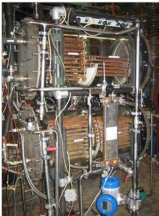
Fig. 3-19: Photograph of the test rig at TU Berlin
