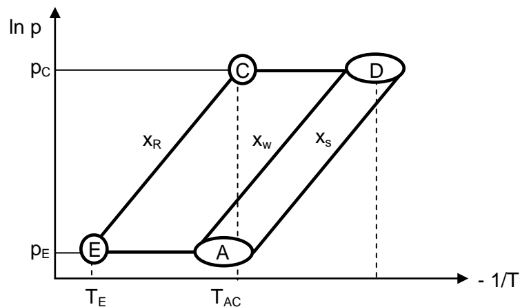
Fig. 1-13: Absorption heat pump cycle in the \ln p - 1/T -diagram
