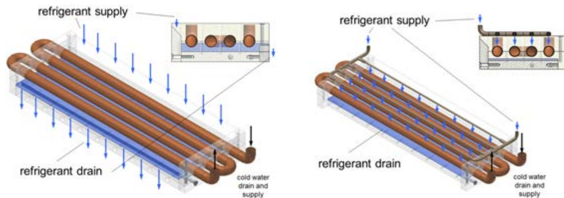
Fig. 3-9: Comparison of pool boiling at a low filling level (left) versus falling film evaporation (right) as investigated in the SORCOOL project at Fraunhofer ISE.
