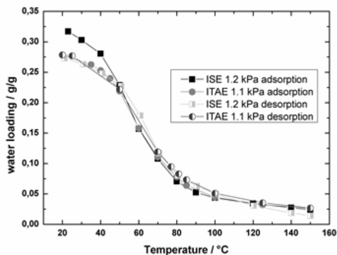
Fig. 3-15: Comparison of 1.1 kPa and 1.2 kPa adsorption/desorption isobars on a SAPO-34 sample. ISE measurements have been performed in an open flow system.
