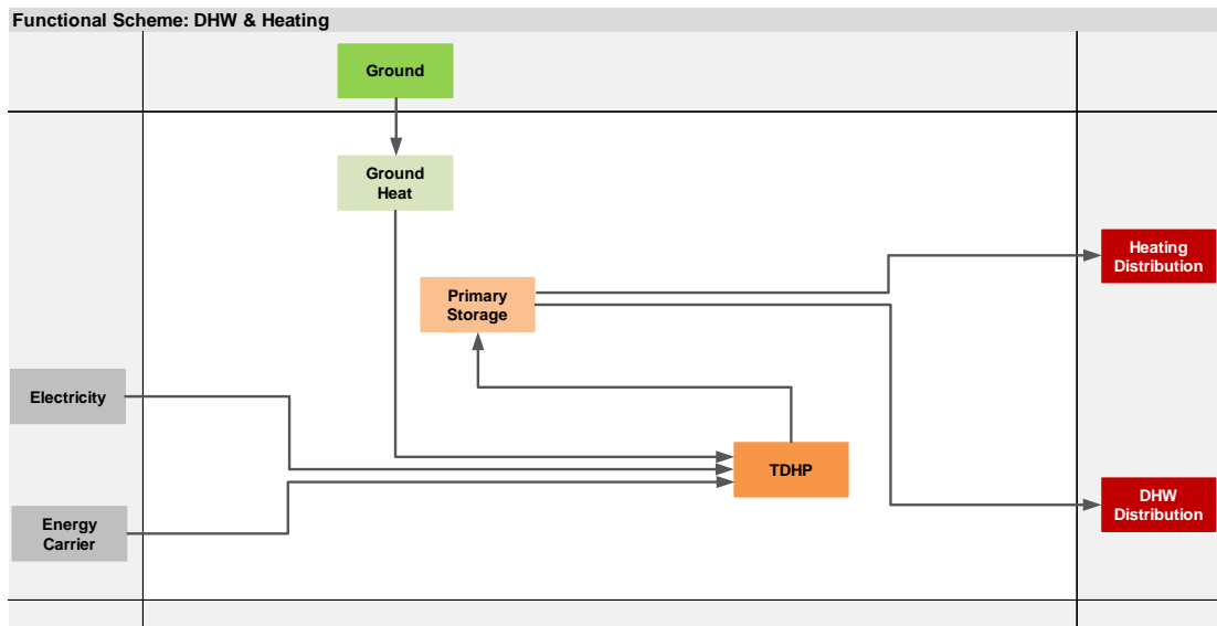
Fig. 5-7: Example of Energy Flow Chart. Winter season: Heating and DHW functional scheme of a plant installed in the brewery’s storehouse in Graz (A) - Source: TU Graz
