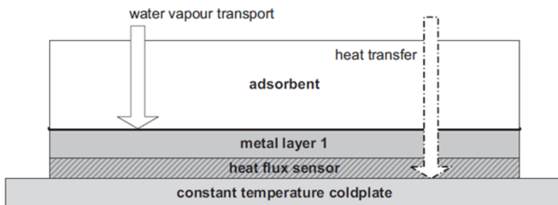
Fig. 3-5: Integration of the sample inside the testing chamber.
