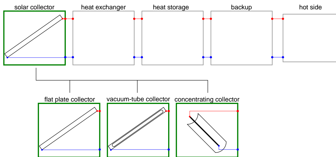
Fig. 4-7: Solar sub-system: options for the solar collector
