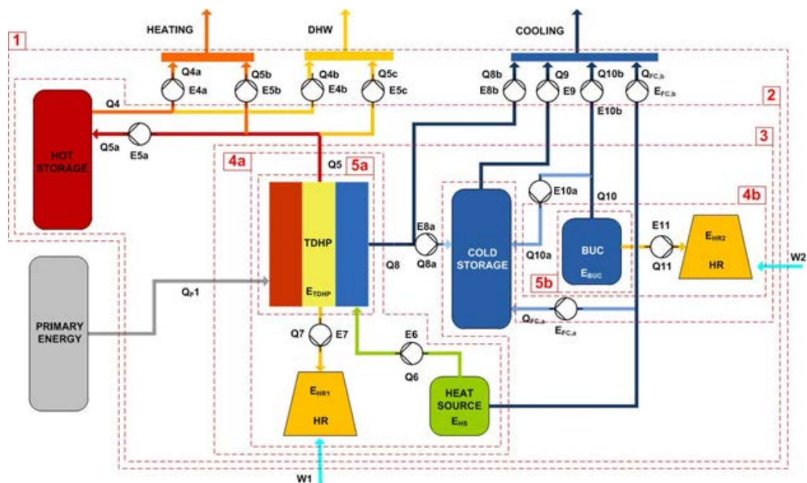
Fig. 2-6 System boundaries and energy flows of a DFHC&C-system
