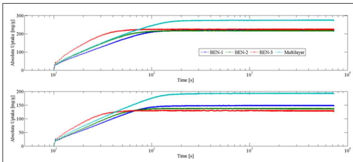
Fig. 3-6: Dynamic evolution of the absolute uptake of the four tested samples: in the upper part after desorption against the vacuum pump, in the lower part after desorption against the condenser @ 30°C.
