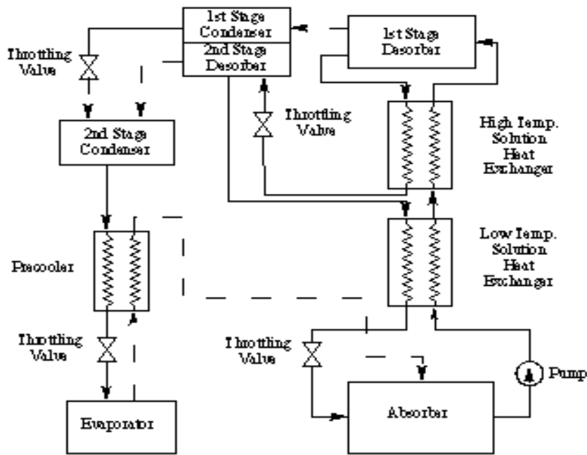
Fig. 1-10: Double effect absorption machine
