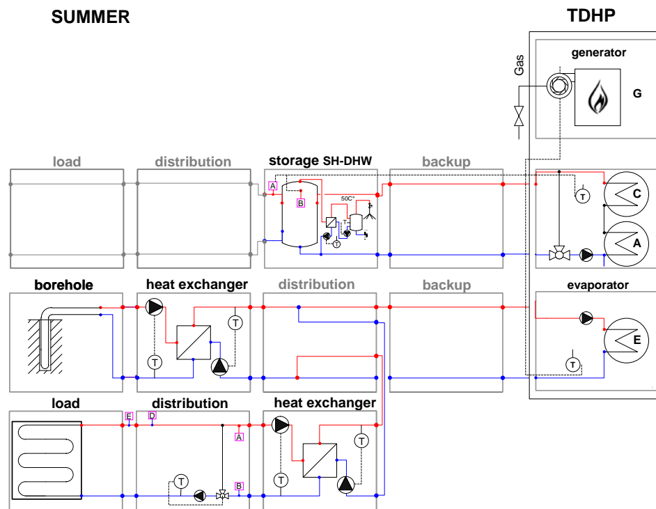
Fig. 5-4: Hydronic representation of a plant installed in the brewery’s storehouse in Graz (A) - summer season: Cooling and DHW functional scheme Source: TU Graz
