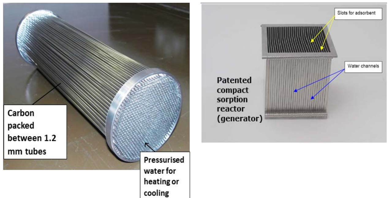
Fig. 1-8: Adsorbers developed at University of Warwick, UK
