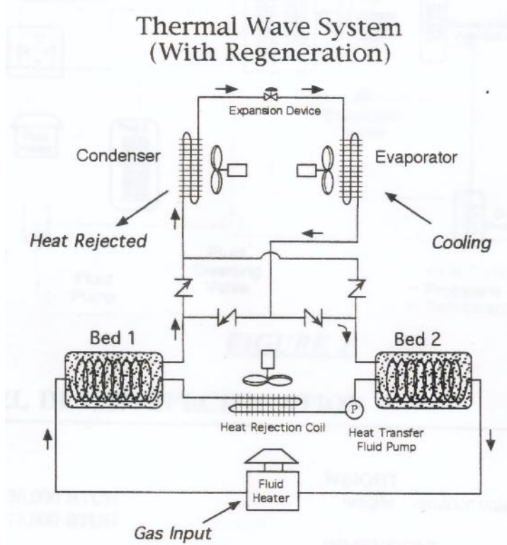
Fig. 1-11: Thermal wave adsorption heat pump patented by Shelton. - Wave Air Corporation, 1993. Solid-Sorption Gas Heat Pump: Technology and market description, internal report, August 1993.
