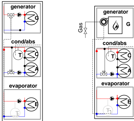
Fig. 4-6: Indirect (left) and direct fired (right) sorption heat pump.
