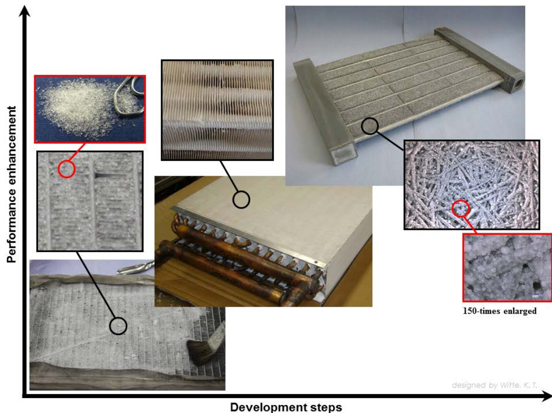
Fig. 3-2: Different evolution steps of the performance enhancement in adsorber development: Packed-bed heat exchanger (left), binder based dip-coated lamella heat exchanger (centre) and direct crystallisation connection of the sorbent (right) on 3D-metal structure heat exchanger. Source (Schossig P. 2011)
