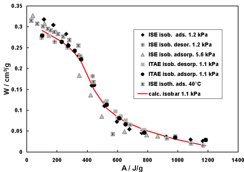
Fig. 3-18: Transformation of equilibrium point for water /SAPO-34 according to Dubinin's theory.
