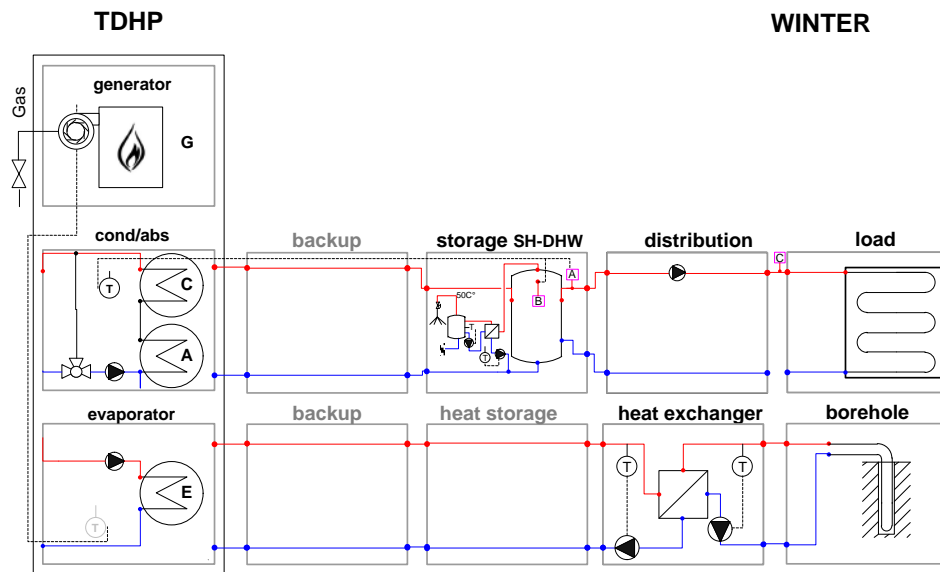
Fig. 5-5: Hydronic representation of a plant installed in the brewery's storehouse in Graz (A) - winter season: Heating and DHW functional scheme. Source: TU Graz
