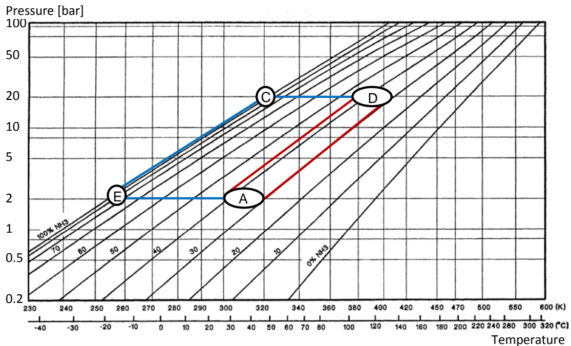
Fig. 1-17: Absorption heat pump cycle in the \ln p-1/T -diagram of \text{NH}_3/\text{water} (Ziegler 1984)
