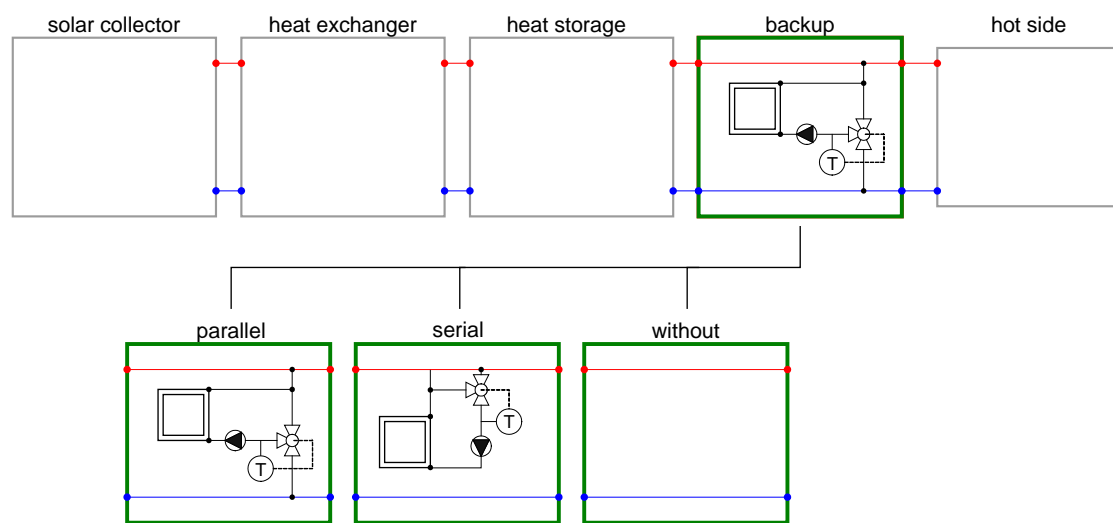
Fig. 4-11: Solar sub-system: options for the integration of the backup-heater.
