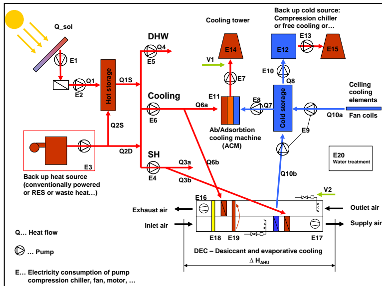
Fig. 4-1: Max-system representation from IEA-SHC Task 38
