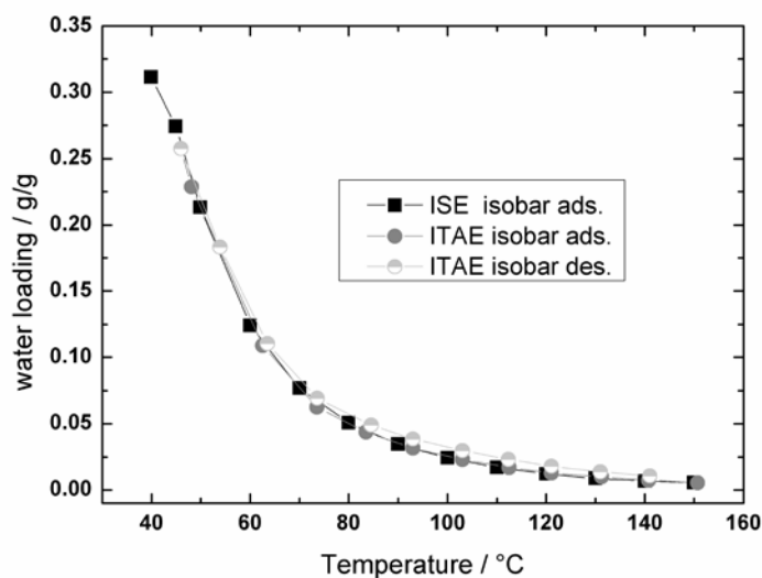
Fig. 3-14: Comparison of isobar adsorption and desorption measurements for Silica Gel 127 B at 5.6 kPa.
