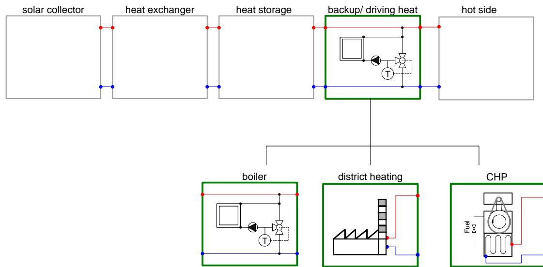
Fig. 4-10: Driving heat sources: Boiler, District heating, and Heat from co-generation systems.
