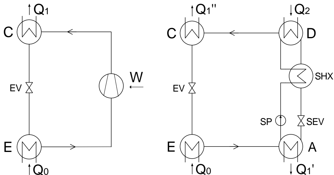
Fig. 1-12: Compression (left) and absorption (right) heat pump cycle
