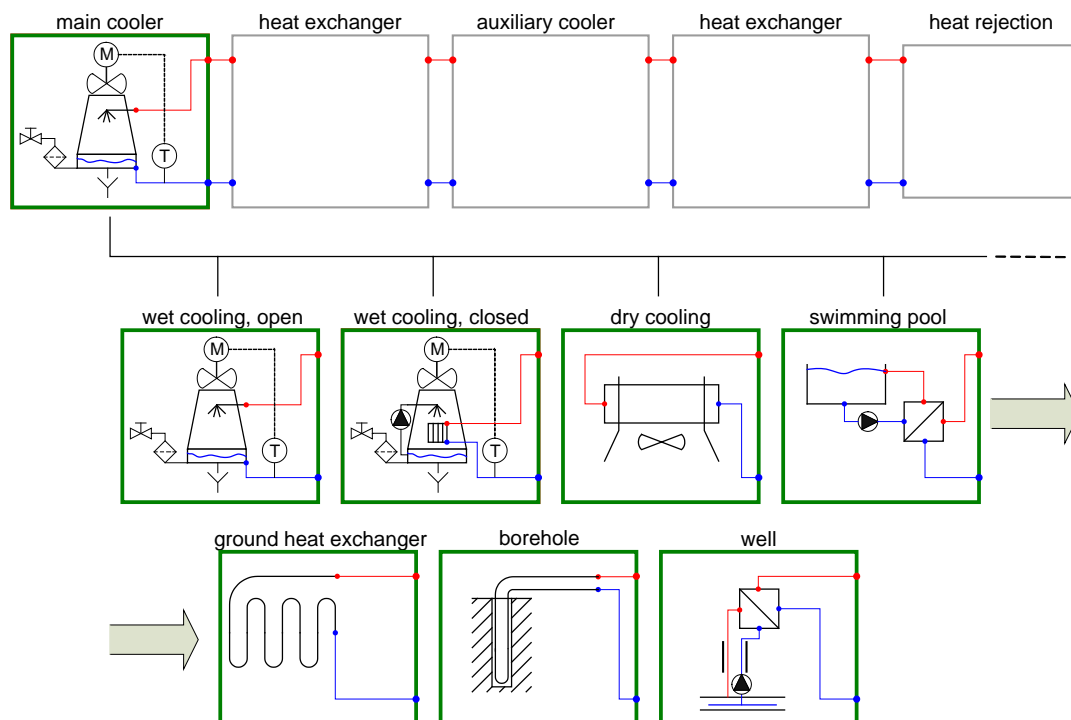
Fig. 4-12: Heat rejection sub-system: open and closed wet and dry cooling towers and alternative heat sinks.
