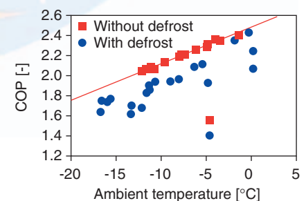
Figure 18: CO 2 heat pump in field test
