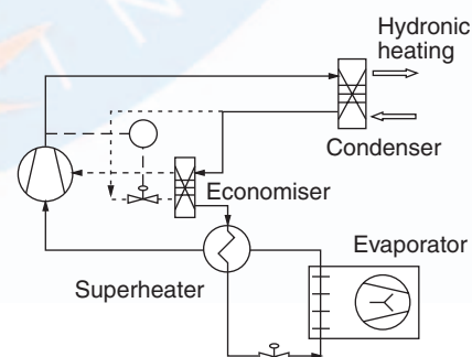
Figure 23: Two-stage dual compressor system for retrofit application
