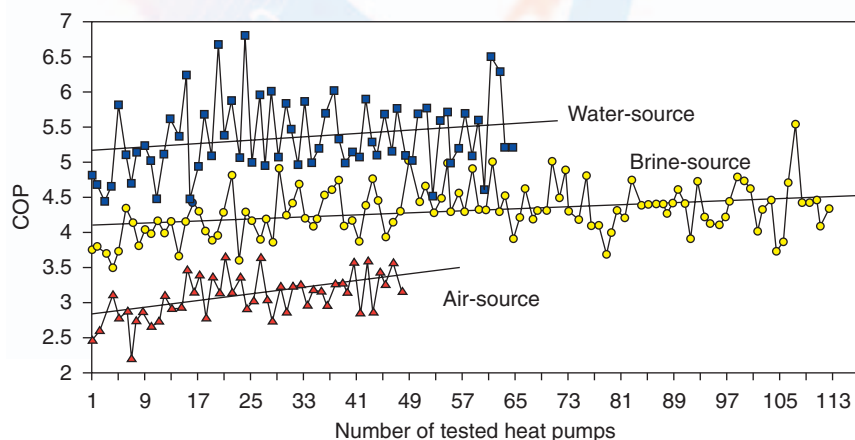
Figure 9: Development of COP (source: Töss)
