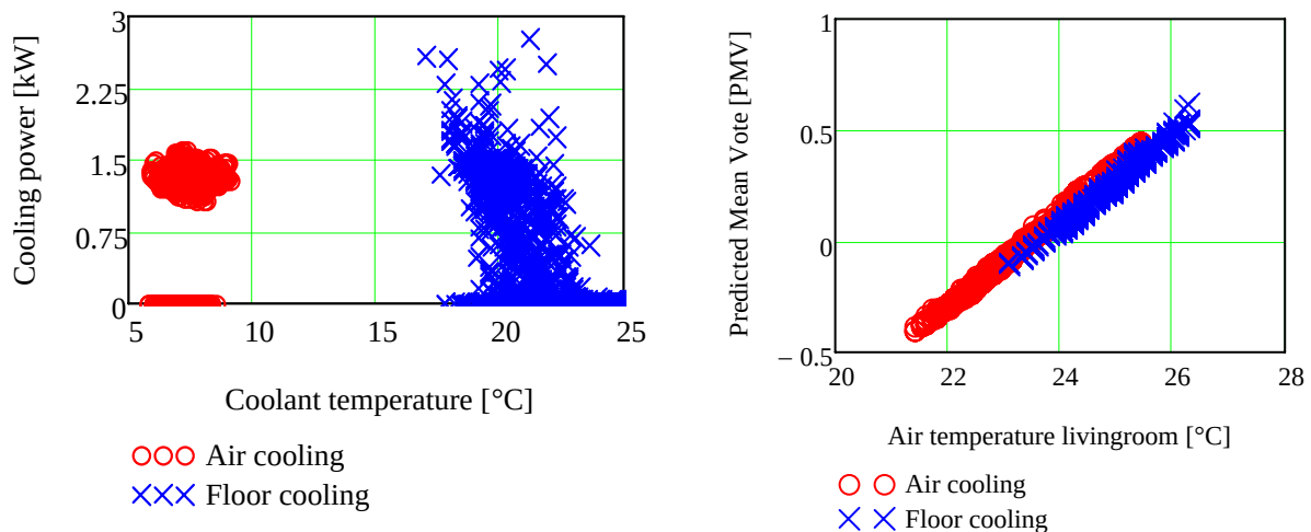
Figure 11: Cooling power versus chilled water temperature during day time
