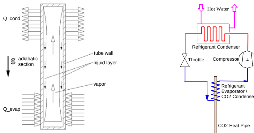
Figure 2: Working principle of a heat pipe (two-phase thermosyphon) and heat pump system layout
