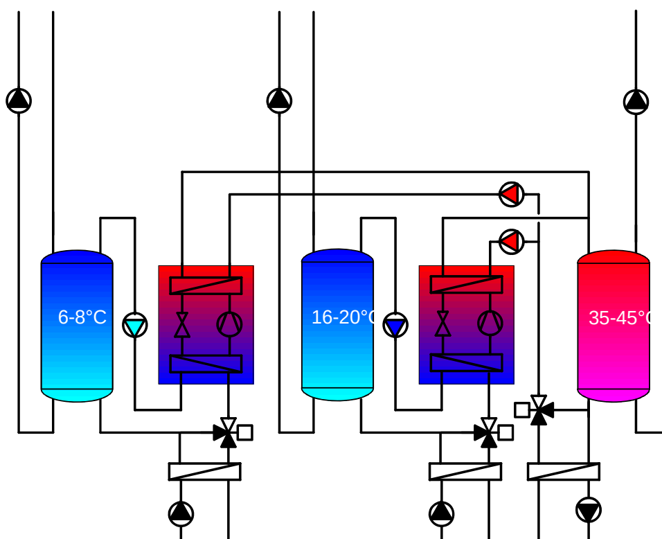
Figure 9: Low-Exergy Air Conditioning System
