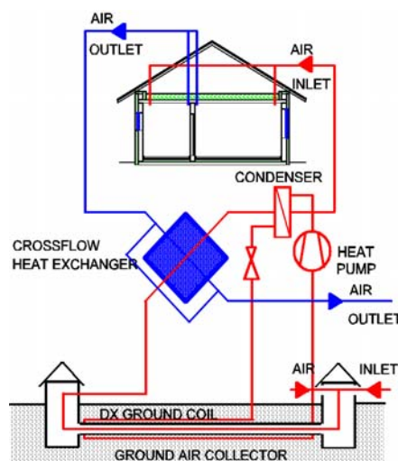
Figure 4: System with Air/Ground Collector, Heat Exchanger and DX/Air Heat Pump
