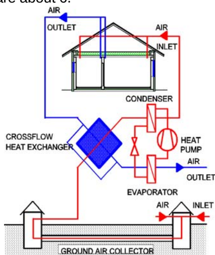
Figure 3: System with Air/Ground Collector, Heat Exchanger and Air/Air Heat Pump
