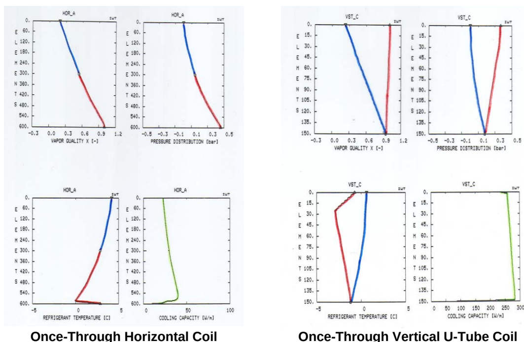
Figure 1: Vapor Quality, Pressure, Temperature, Heat Extraction Rate
