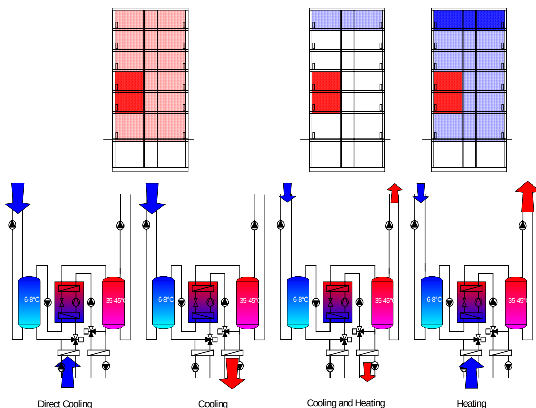
Figure 6: Ground Source Air Conditioning System for an Office Building
