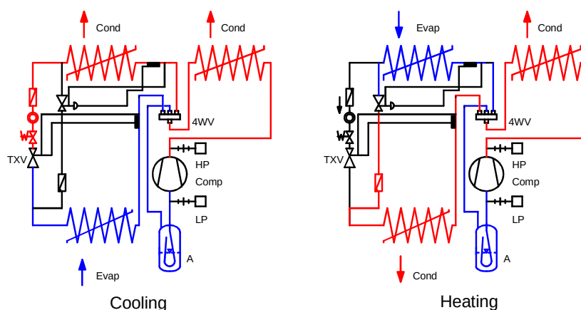
Figure 5: Reversible Double Condenser Heat Pump Unit
