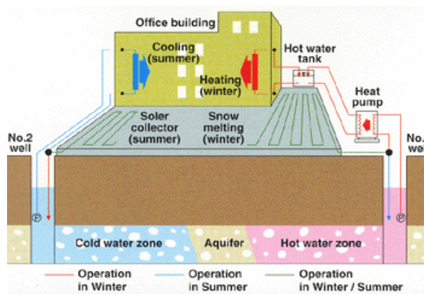
Figure 8: Aquifer System
