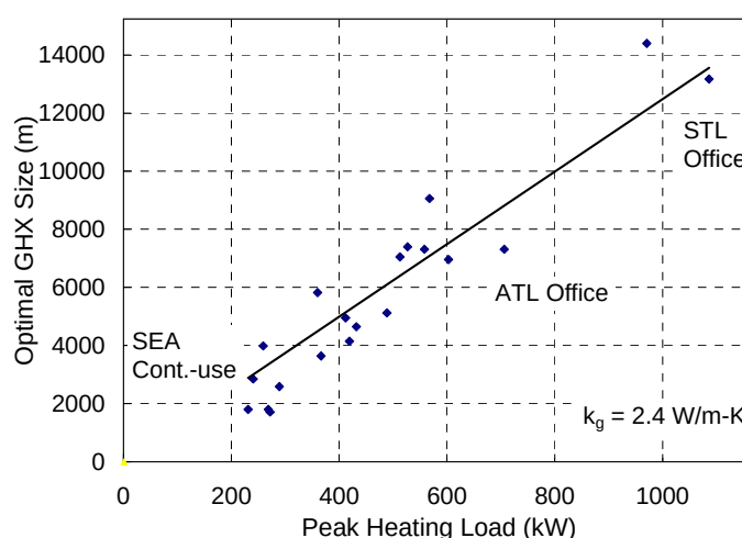
Figure 2. Optimal GHX size as a function of peak heating load for each scenario.
