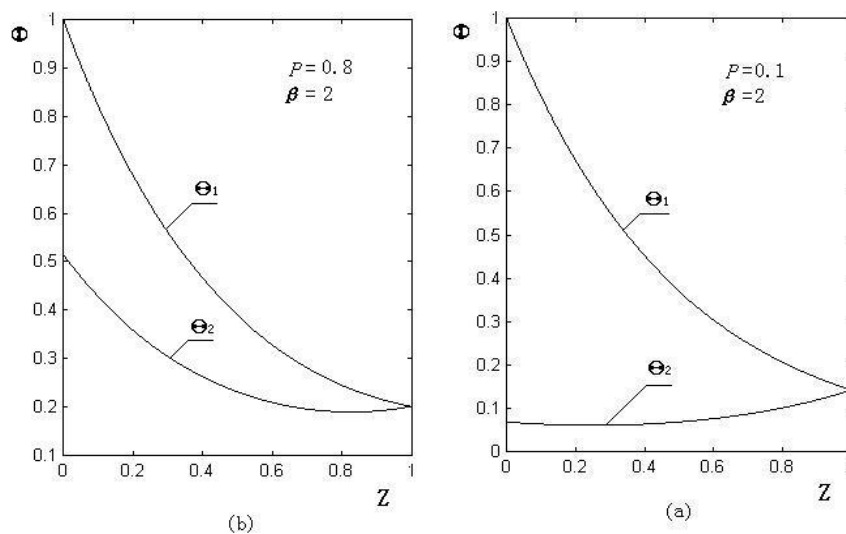
Figure 2: Fluid temperature profiles along the borehole depth
