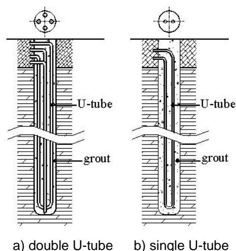
Figure 1: Schematic diagram of boreholes in the vertical GHE
