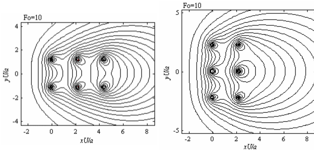
Figure 4: Isotherms of borehole fields with different configurations to the advection direction
