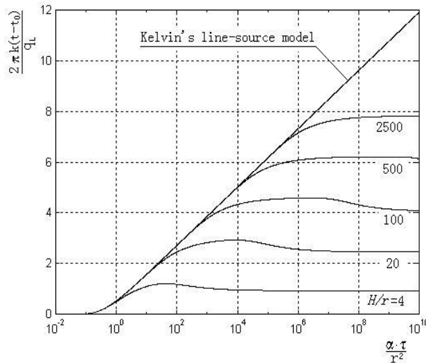
Figure 3: Temperature responses of a line source in 1-D and 2-D models
