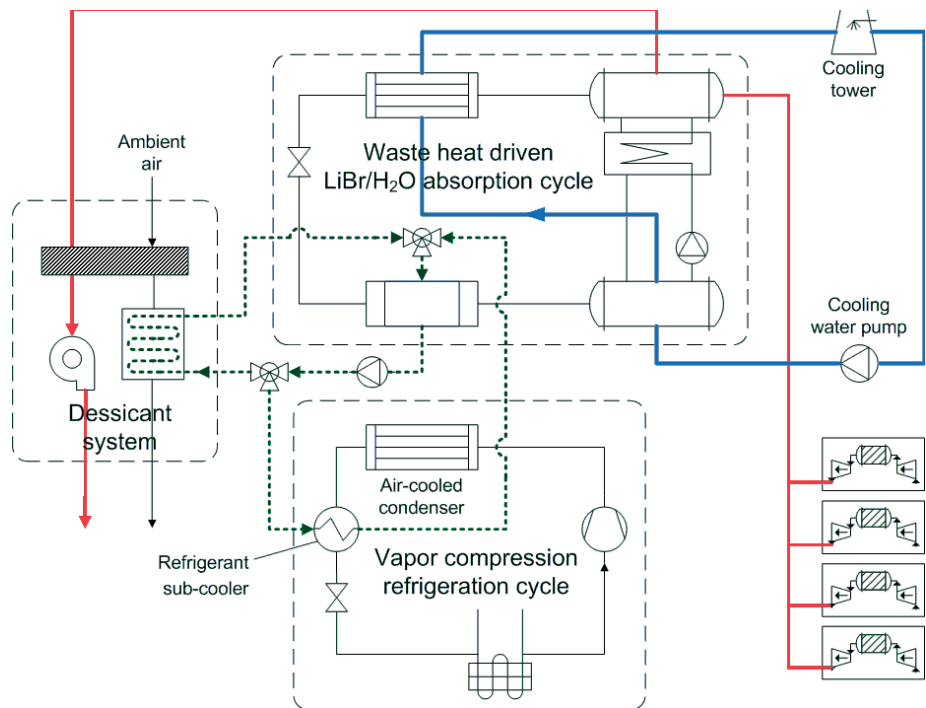
Figure 3. PureComfort™ 240M Integration with Supermarket System
