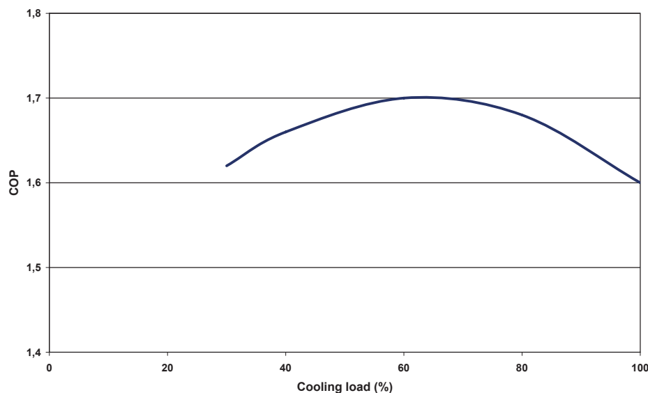
Figure 3. Partial loading characteristics
