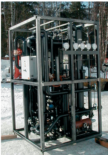
Figure 2. Double lift ThermoChiller prior to installation
