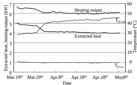
Fig. 10. Extracted heat, heating output and temperatures of T_{f1-in} and T_{f2-out} obtained from the first season's operation
